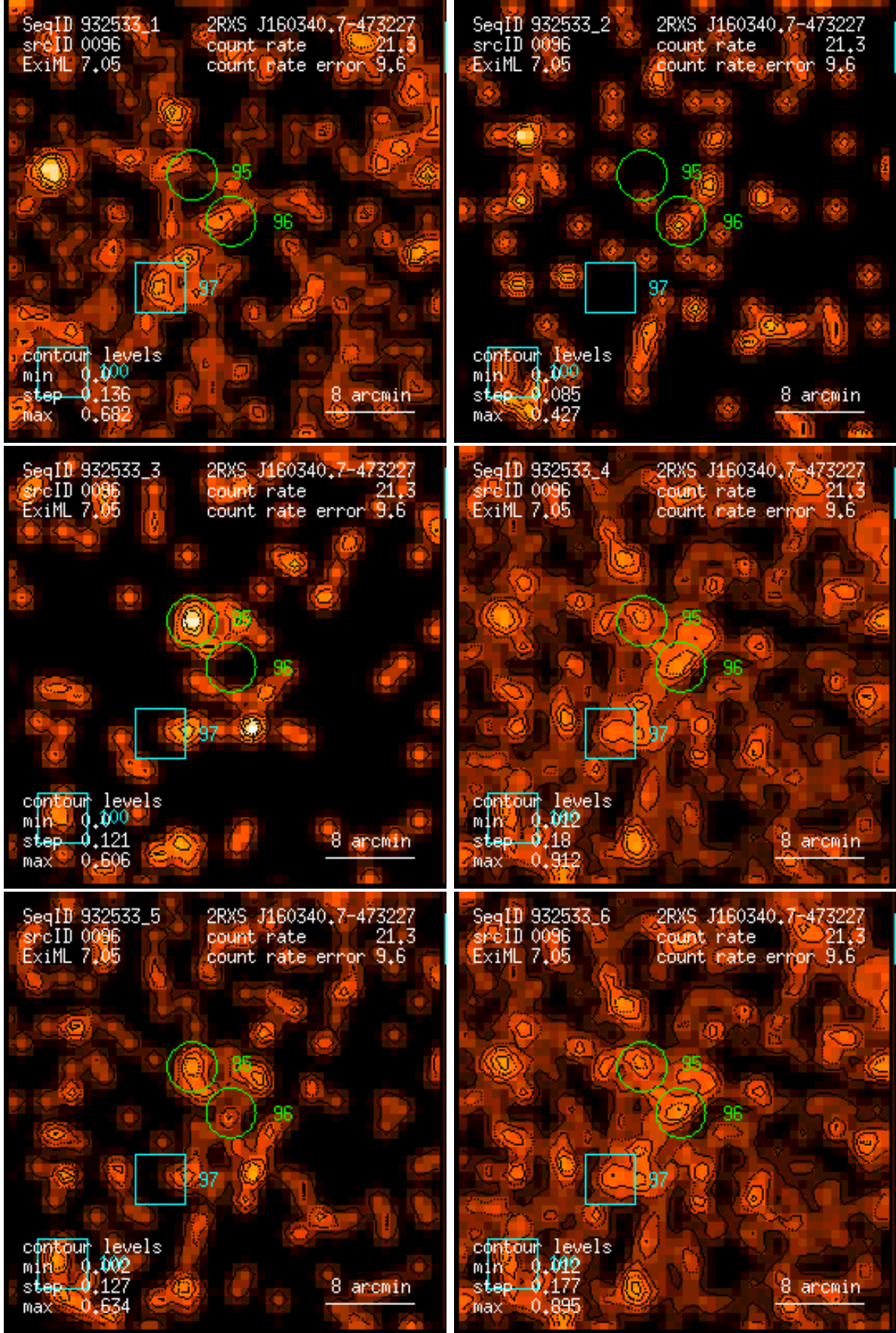
Figure 96: RASS 932533: detection 0096: band rate images, Gaussian filter: (1) PSPC channels 11 – 41, (2) 52 – 90, (3) 91 – 201, (4) 11 – 235, (5) 52 – 201, (6) 11 – 201. Broad band rates in counts/ks. Band rate contour levels in counts/ks/arcmin 2 .
