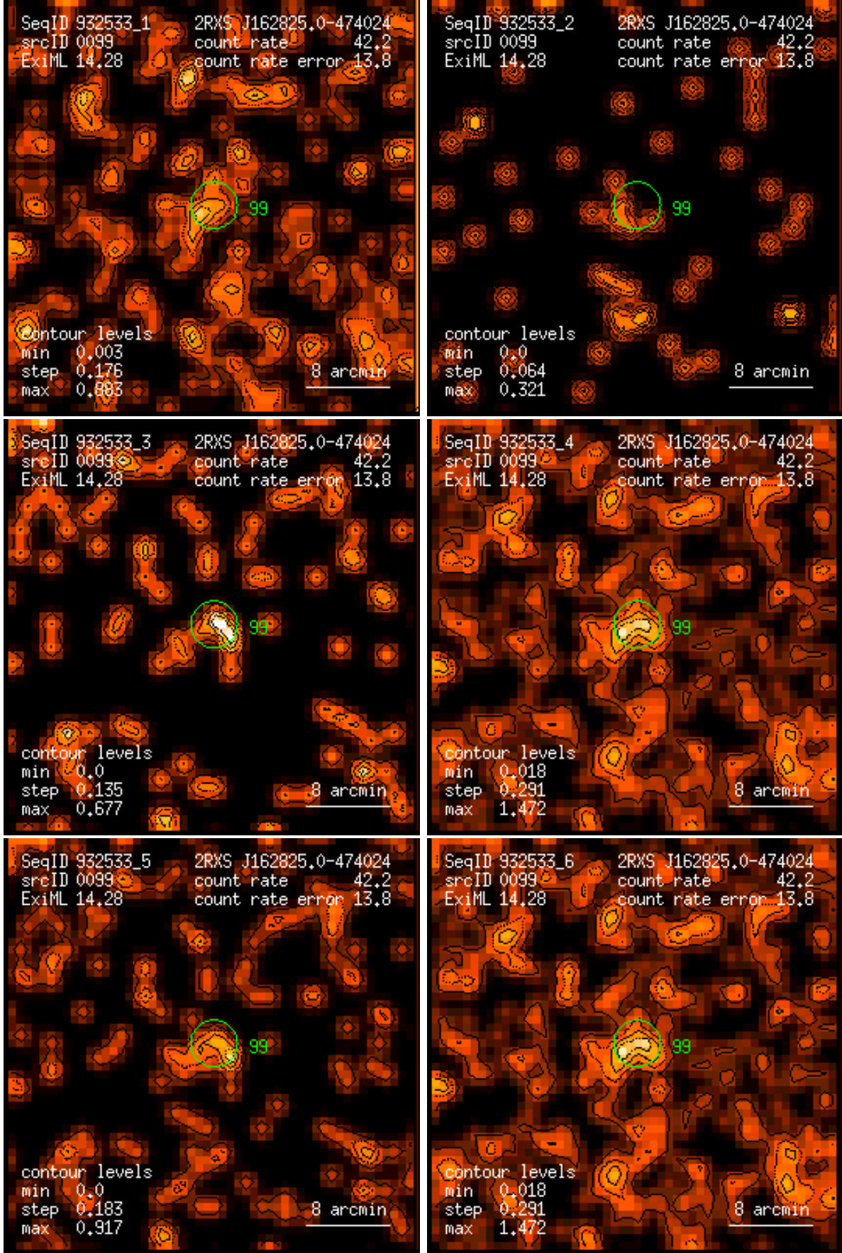
Figure 99: RASS 932533: detection 0099: band rate images, Gaussian filter: (1) PSPC channels 11 – 41, (2) 52 – 90, (3) 91 – 201, (4) 11 – 235, (5) 52 – 201, (6) 11 – 201. Broad band rates in counts/ks. Band rate contour levels in counts/ks/arcmin 2 .
