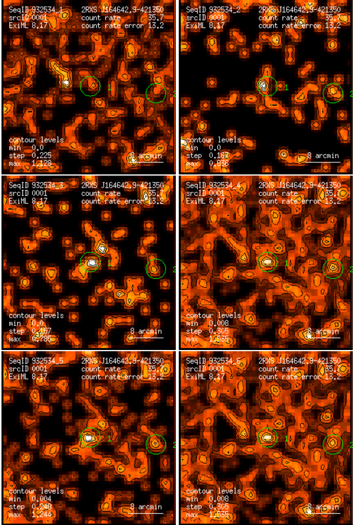
Figure 1: RASS 932534: detection 0001: band rate images, Gaussian filter: (1) PSPC channels 11 – 41, (2) 52 – 90, (3) 91 – 201, (4) 11 – 235, (5) 52 – 201, (6) 11 – 201. Broad band rates in counts/ks. Band rate contour levels in counts/ks/arcmin 2 .
