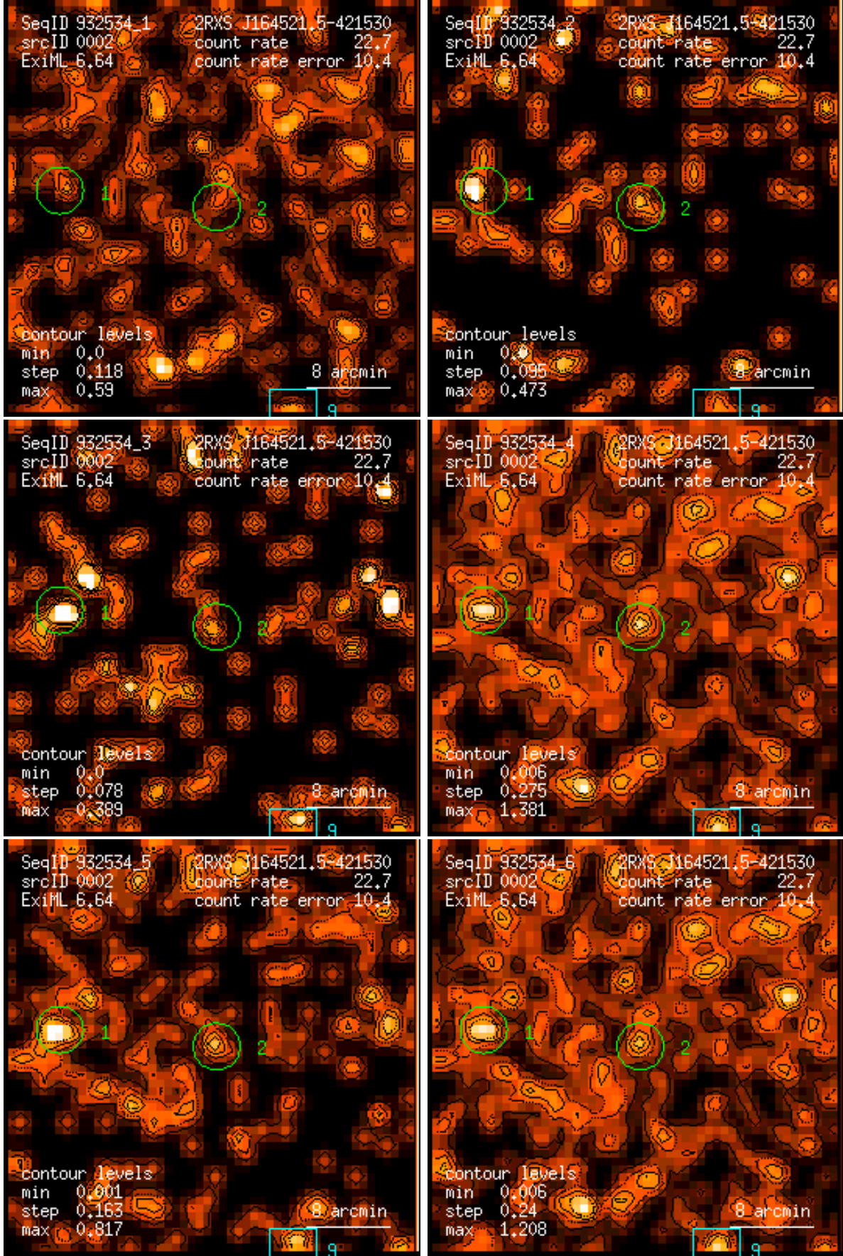
Figure 2: RASS 932534: detection 0002: band rate images, Gaussian filter: (1) PSPC channels 11 – 41, (2) 52 – 90, (3) 91 – 201, (4) 11 – 235, (5) 52 – 201, (6) 11 – 201. Broad band rates in counts/ks. Band rate contour levels in counts/ks/arcmin 2 .
