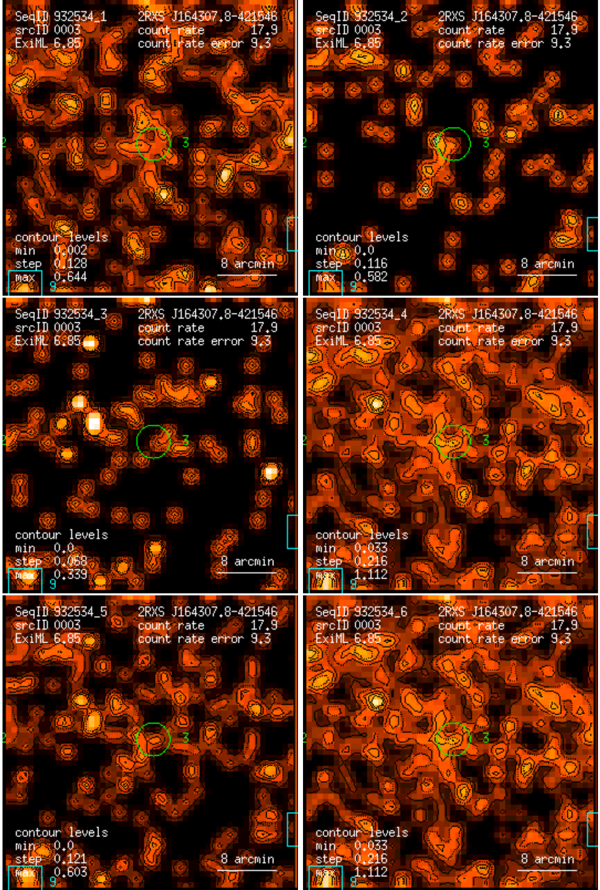
Figure 3: RASS 932534: detection 0003: band rate images, Gaussian filter: (1) PSPC channels 11 – 41, (2) 52 – 90, (3) 91 – 201, (4) 11 – 235, (5) 52 – 201, (6) 11 – 201. Broad band rates in counts/ks. Band rate contour levels in counts/ks/arcmin 2 .
