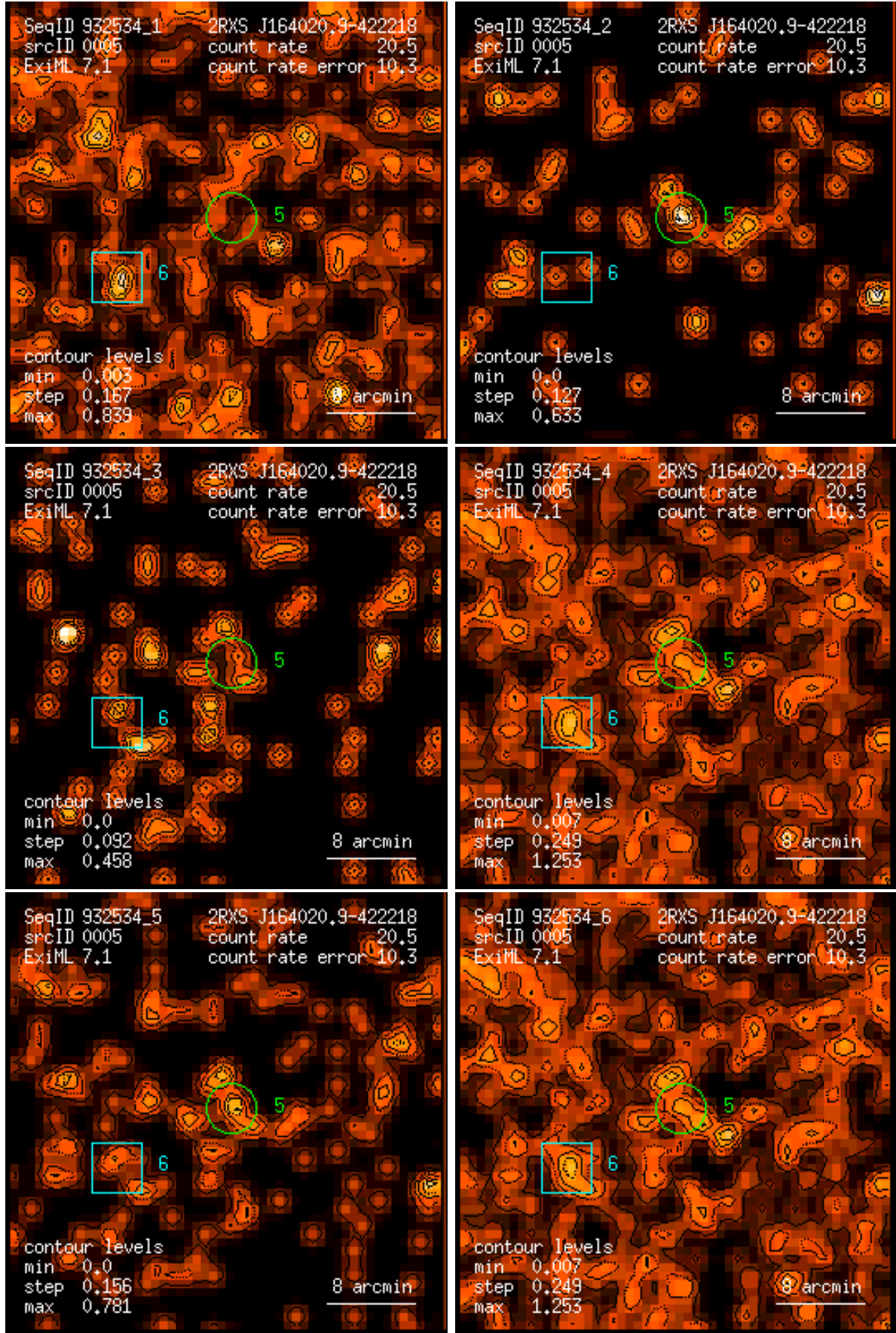
Figure 5: RASS 932534: detection 0005: band rate images, Gaussian filter: (1) PSPC channels 11 – 41, (2) 52 – 90, (3) 91 – 201, (4) 11 – 235, (5) 52 – 201, (6) 11 – 201. Broad band rates in counts/ks. Band rate contour levels in counts/ks/arcmin 2 .
