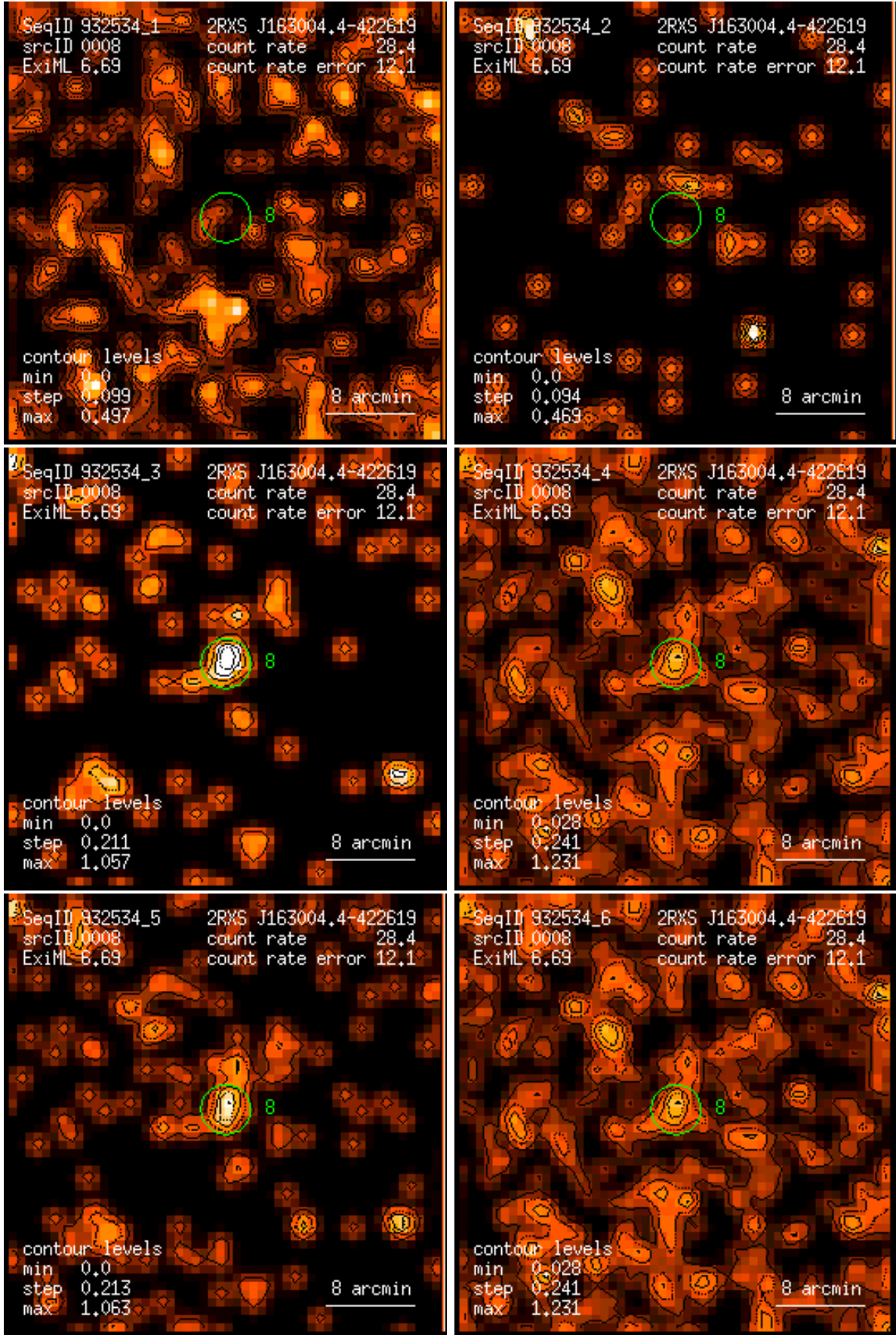
Figure 8: RASS 932534: detection 0008: band rate images, Gaussian filter: (1) PSPC channels 11 – 41, (2) 52 – 90, (3) 91 – 201, (4) 11 – 235, (5) 52 – 201, (6) 11 – 201. Broad band rates in counts/ks. Band rate contour levels in counts/ks/arcmin 2 .
