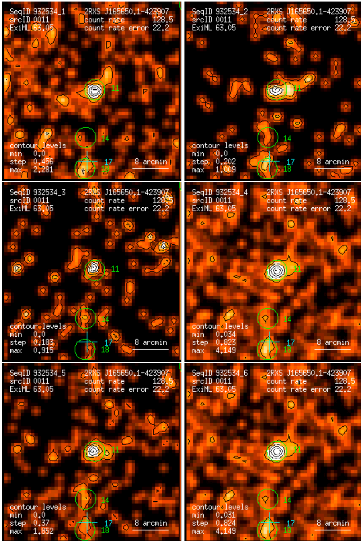
Figure 11: RASS 932534: detection 0011: band rate images, Gaussian filter: (1) PSPC channels 11 – 41, (2) 52 – 90, (3) 91 – 201, (4) 11 – 235, (5) 52 – 201, (6) 11 – 201. Broad band rates in counts/ks. Band rate contour levels in counts/ks/arcmin 2 .
