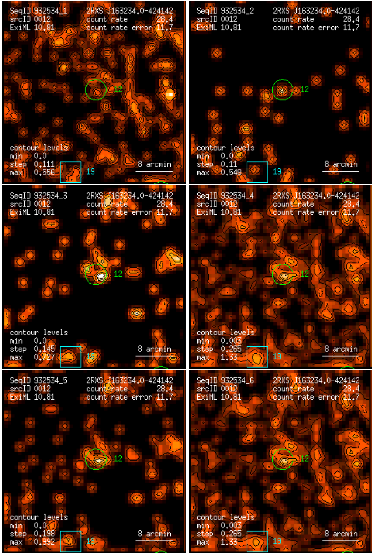
Figure 12: RASS 932534: detection 0012: band rate images, Gaussian filter: (1) PSPC channels 11 – 41, (2) 52 – 90, (3) 91 – 201, (4) 11 – 235, (5) 52 – 201, (6) 11 – 201. Broad band rates in counts/ks. Band rate contour levels in counts/ks/arcmin 2 .
