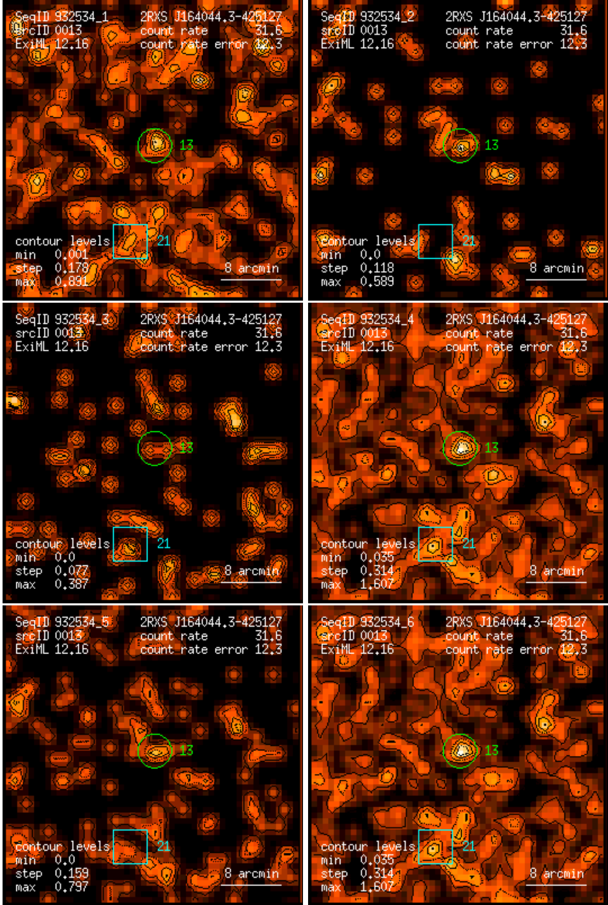
Figure 13: RASS 932534: detection 0013: band rate images, Gaussian filter: (1) PSPC channels 11 – 41, (2) 52 – 90, (3) 91 – 201, (4) 11 – 235, (5) 52 – 201, (6) 11 – 201. Broad band rates in counts/ks. Band rate contour levels in counts/ks/arcmin 2 .
