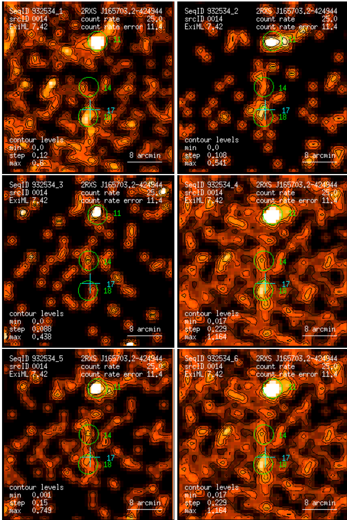
Figure 14: RASS 932534: detection 0014: band rate images, Gaussian filter: (1) PSPC channels 11 – 41, (2) 52 – 90, (3) 91 – 201, (4) 11 – 235, (5) 52 – 201, (6) 11 – 201. Broad band rates in counts/ks. Band rate contour levels in counts/ks/arcmin 2 .
