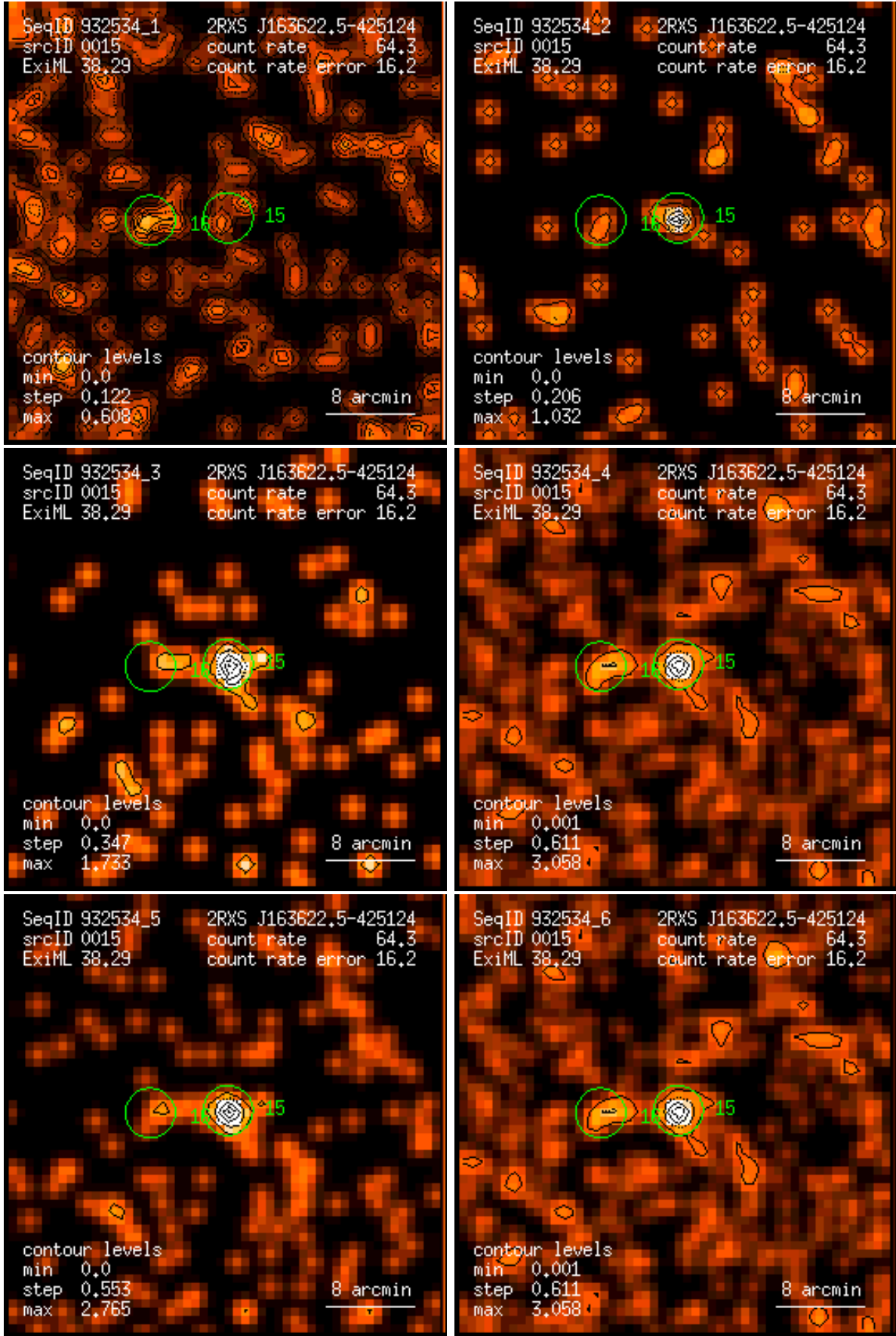
Figure 15: RASS 932534: detection 0015: band rate images, Gaussian filter: (1) PSPC channels 11 – 41, (2) 52 – 90, (3) 91 – 201, (4) 11 – 235, (5) 52 – 201, (6) 11 – 201. Broad band rates in counts/ks. Band rate contour levels in counts/ks/arcmin 2 .
