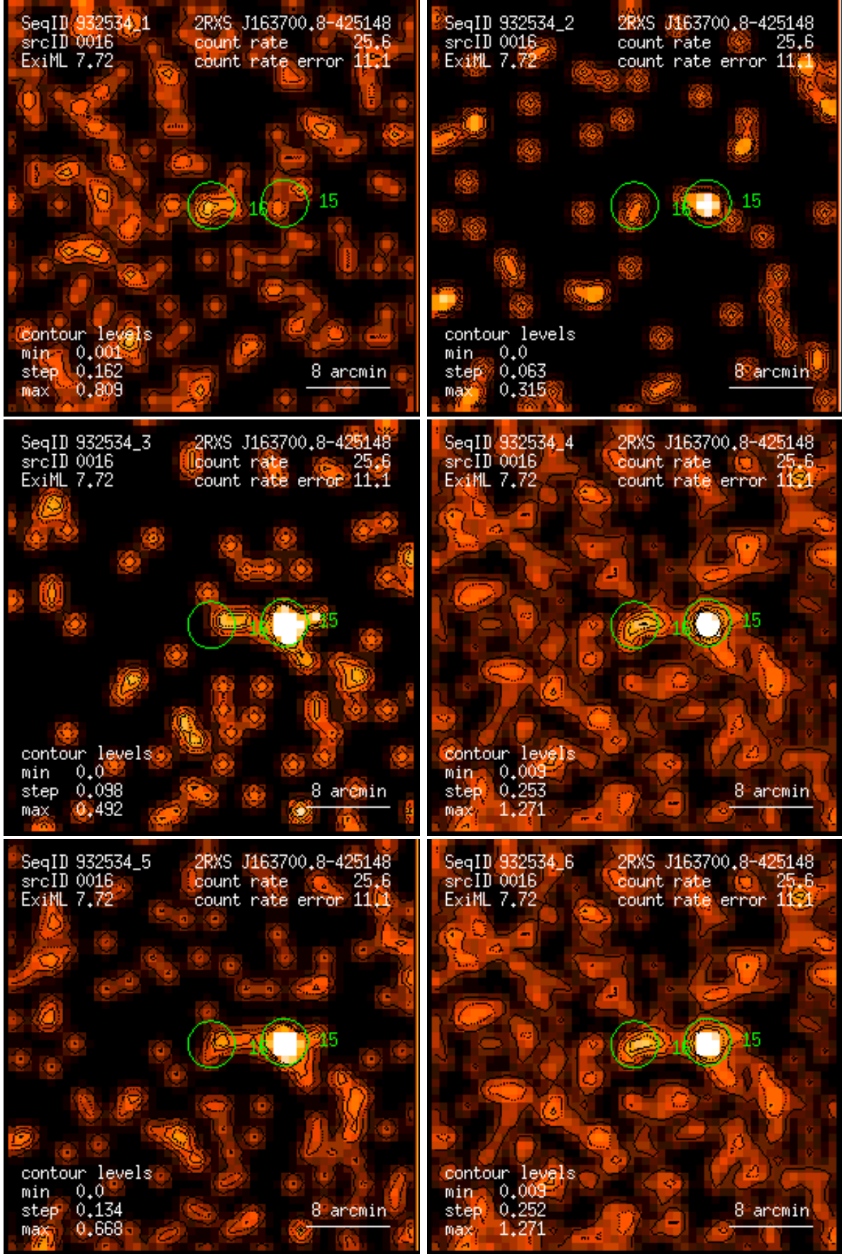
Figure 16: RASS 932534: detection 0016: band rate images, Gaussian filter: (1) PSPC channels 11 – 41, (2) 52 – 90, (3) 91 – 201, (4) 11 – 235, (5) 52 – 201, (6) 11 – 201. Broad band rates in counts/ks. Band rate contour levels in counts/ks/arcmin 2 .
