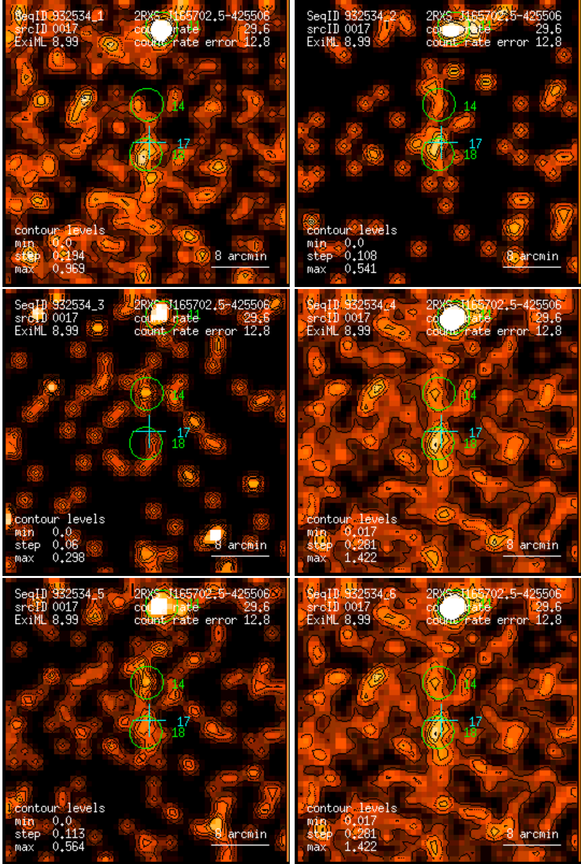
Figure 17: RASS 932534: detection 0017: band rate images, Gaussian filter: (1) PSPC channels 11 – 41, (2) 52 – 90, (3) 91 – 201, (4) 11 – 235, (5) 52 – 201, (6) 11 – 201. Broad band rates in counts/ks. Band rate contour levels in counts/ks/arcmin 2 .
