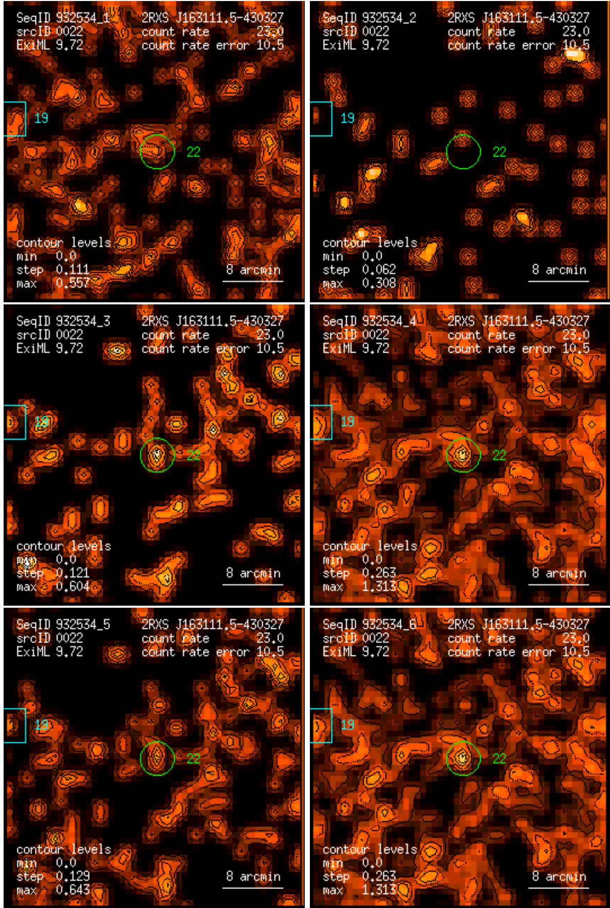
Figure 22: RASS 932534: detection 0022: band rate images, Gaussian filter: (1) PSPC channels 11 – 41, (2) 52 – 90, (3) 91 – 201, (4) 11 – 235, (5) 52 – 201, (6) 11 – 201. Broad band rates in counts/ks. Band rate contour levels in counts/ks/arcmin 2 .
