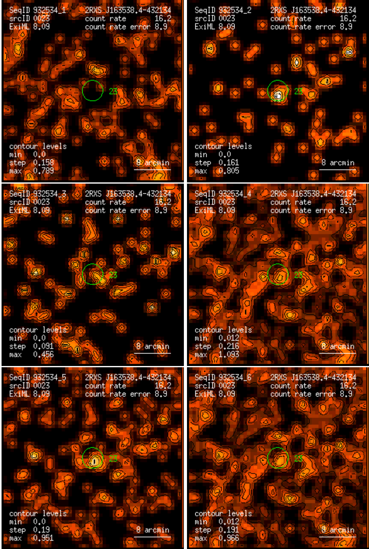
Figure 23: RASS 932534: detection 0023: band rate images, Gaussian filter: (1) PSPC channels 11 – 41, (2) 52 – 90, (3) 91 – 201, (4) 11 – 235, (5) 52 – 201, (6) 11 – 201. Broad band rates in counts/ks. Band rate contour levels in counts/ks/arcmin 2 .
