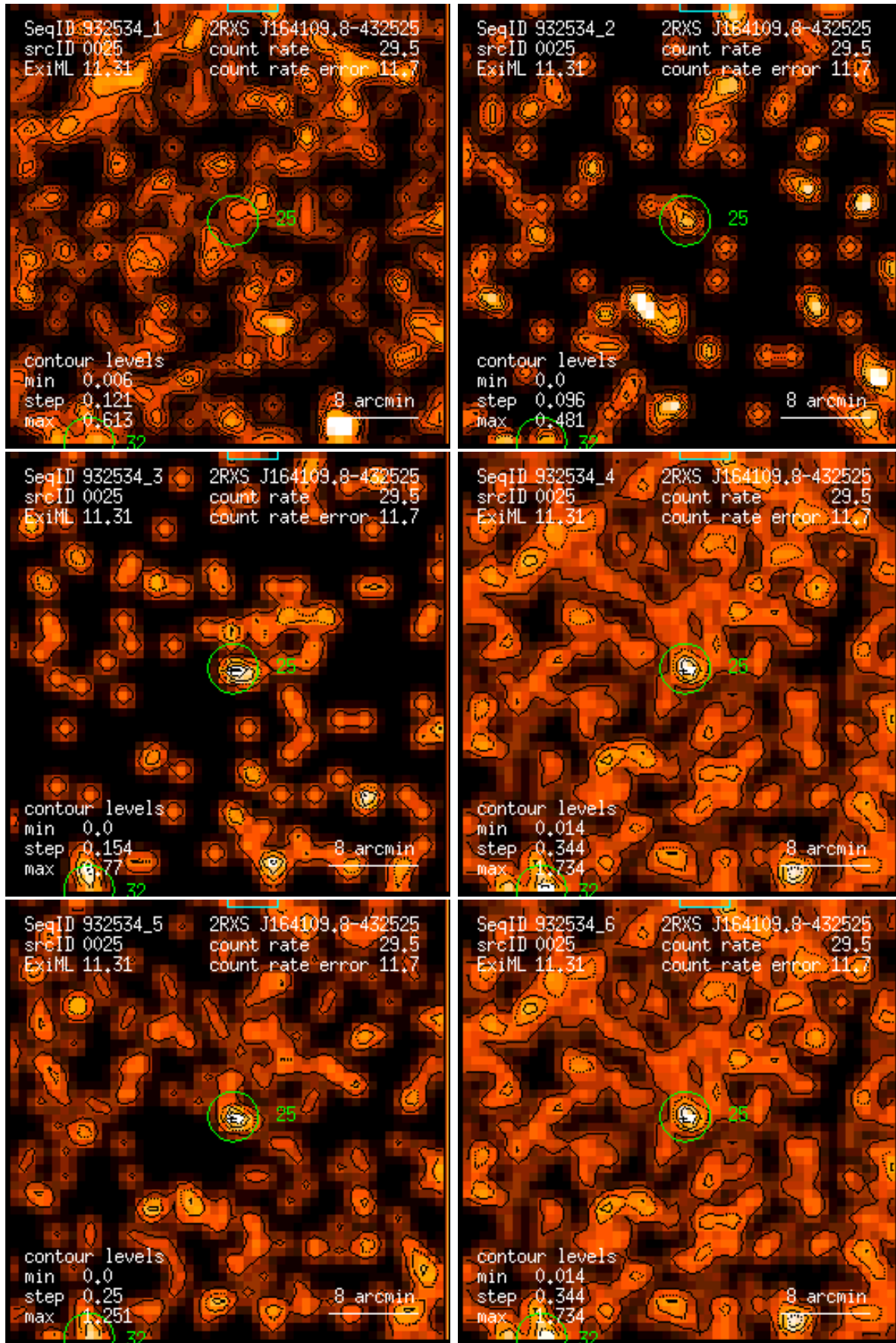
Figure 25: RASS 932534: detection 0025: band rate images, Gaussian filter: (1) PSPC channels 11 – 41, (2) 52 – 90, (3) 91 – 201, (4) 11 – 235, (5) 52 – 201, (6) 11 – 201. Broad band rates in counts/ks. Band rate contour levels in counts/ks/arcmin 2 .
