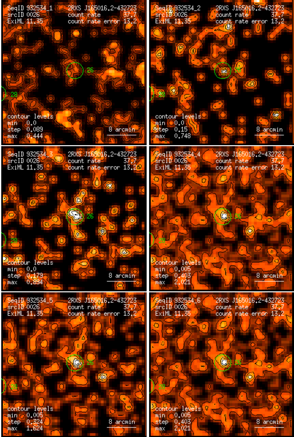
Figure 26: RASS 932534: detection 0026: band rate images, Gaussian filter: (1) PSPC channels 11 – 41, (2) 52 – 90, (3) 91 – 201, (4) 11 – 235, (5) 52 – 201, (6) 11 – 201. Broad band rates in counts/ks. Band rate contour levels in counts/ks/arcmin 2 .
