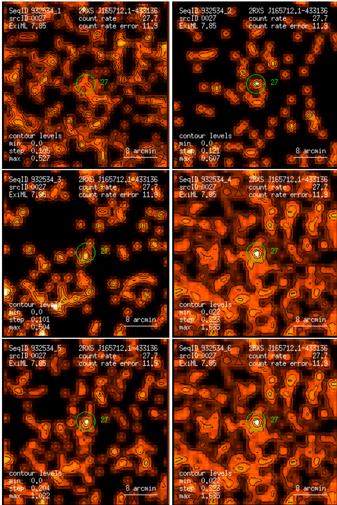
Figure 27: RASS 932534: detection 0027: band rate images, Gaussian filter: (1) PSPC channels 11 – 41, (2) 52 – 90, (3) 91 – 201, (4) 11 – 235, (5) 52 – 201, (6) 11 – 201. Broad band rates in counts/ks. Band rate contour levels in counts/ks/arcmin 2 .
