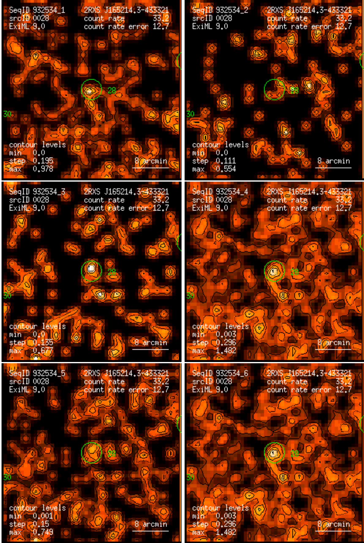
Figure 28: RASS 932534: detection 0028: band rate images, Gaussian filter: (1) PSPC channels 11 – 41, (2) 52 – 90, (3) 91 – 201, (4) 11 – 235, (5) 52 – 201, (6) 11 – 201. Broad band rates in counts/ks. Band rate contour levels in counts/ks/arcmin 2 .
