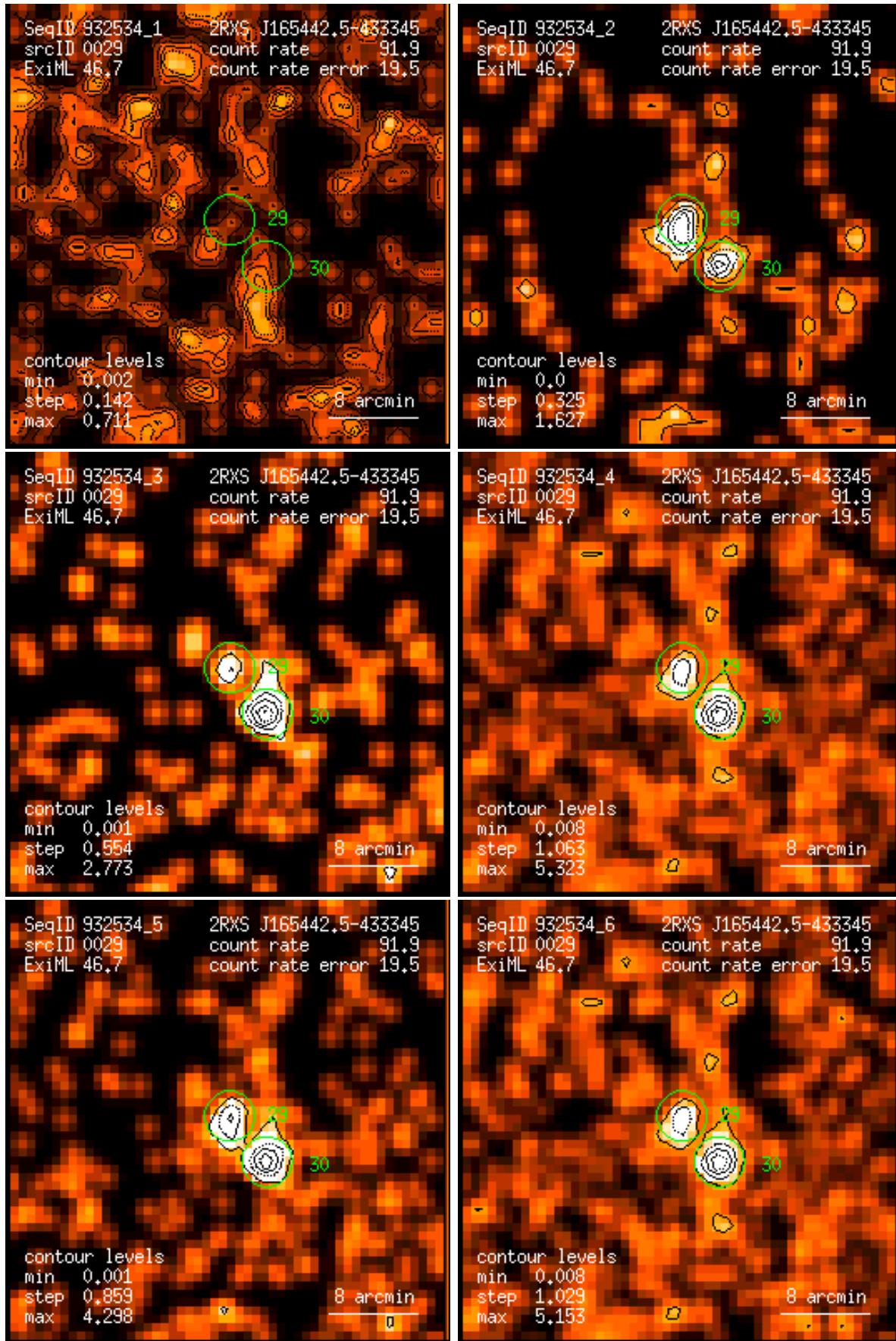
Figure 29: RASS 932534: detection 0029: band rate images, Gaussian filter: (1) PSPC channels 11 – 41, (2) 52 – 90, (3) 91 – 201, (4) 11 – 235, (5) 52 – 201, (6) 11 – 201. Broad band rates in counts/ks. Band rate contour levels in counts/ks/arcmin 2 .
