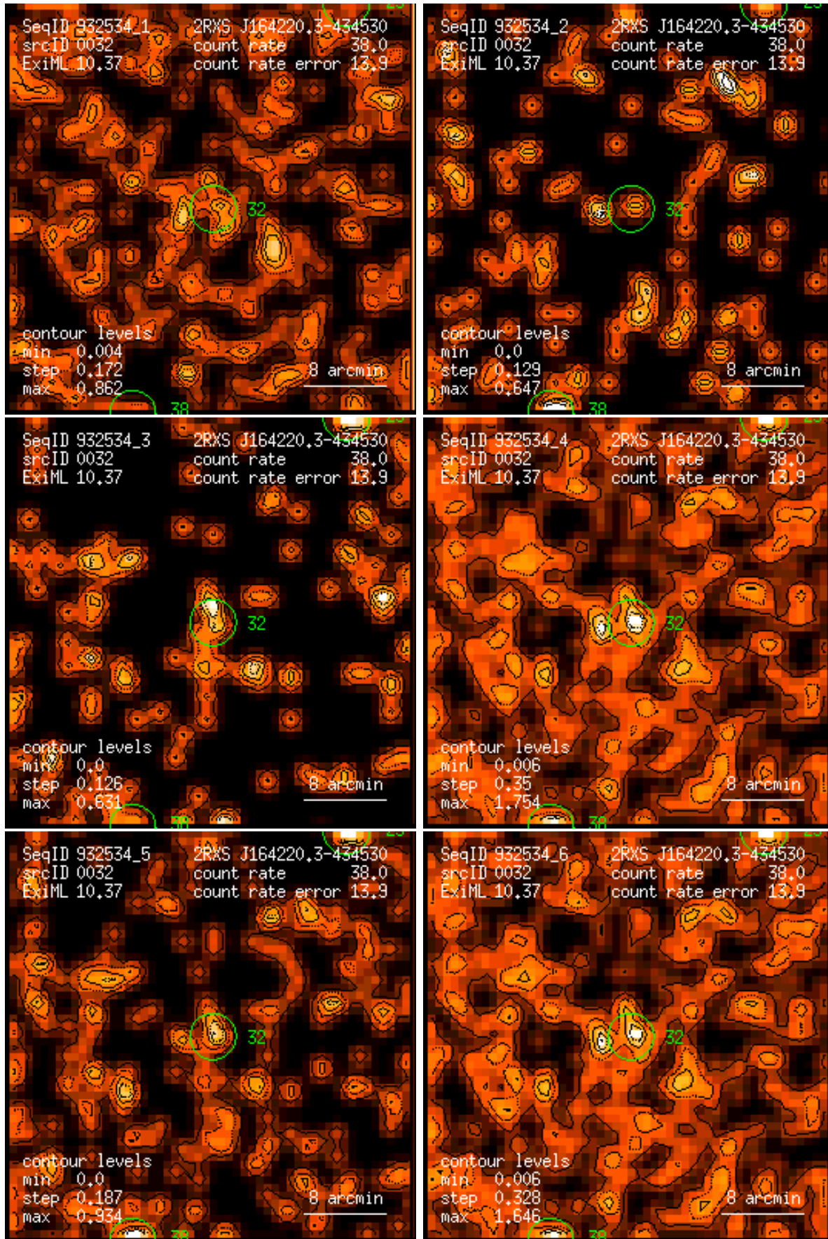
Figure 32: RASS 932534: detection 0032: band rate images, Gaussian filter: (1) PSPC channels 11 – 41, (2) 52 – 90, (3) 91 – 201, (4) 11 – 235, (5) 52 – 201, (6) 11 – 201. Broad band rates in counts/ks. Band rate contour levels in counts/ks/arcmin 2 .
