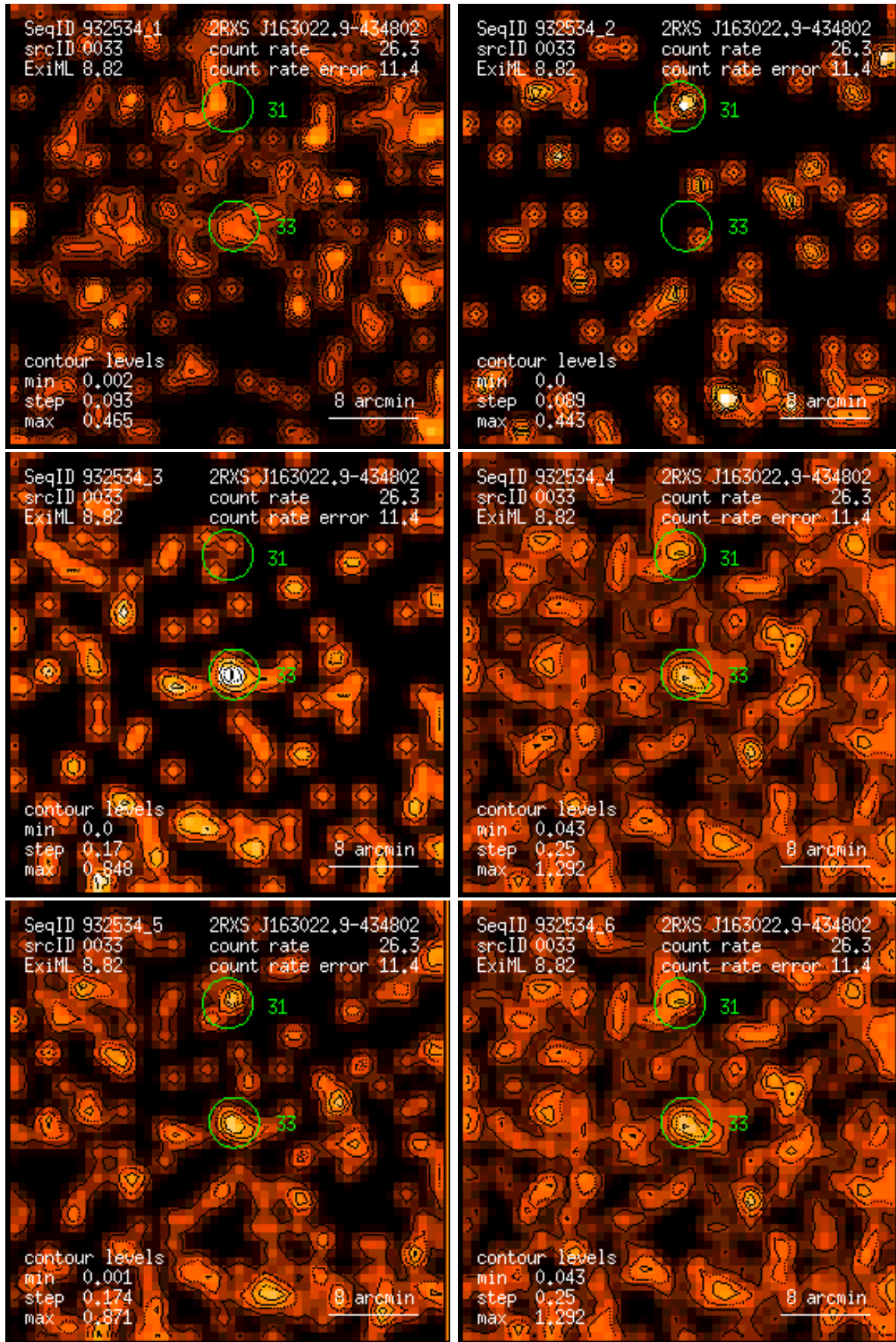
Figure 33: RASS 932534: detection 0033: band rate images, Gaussian filter: (1) PSPC channels 11 – 41, (2) 52 – 90, (3) 91 – 201, (4) 11 – 235, (5) 52 – 201, (6) 11 – 201. Broad band rates in counts/ks. Band rate contour levels in counts/ks/arcmin 2 .
