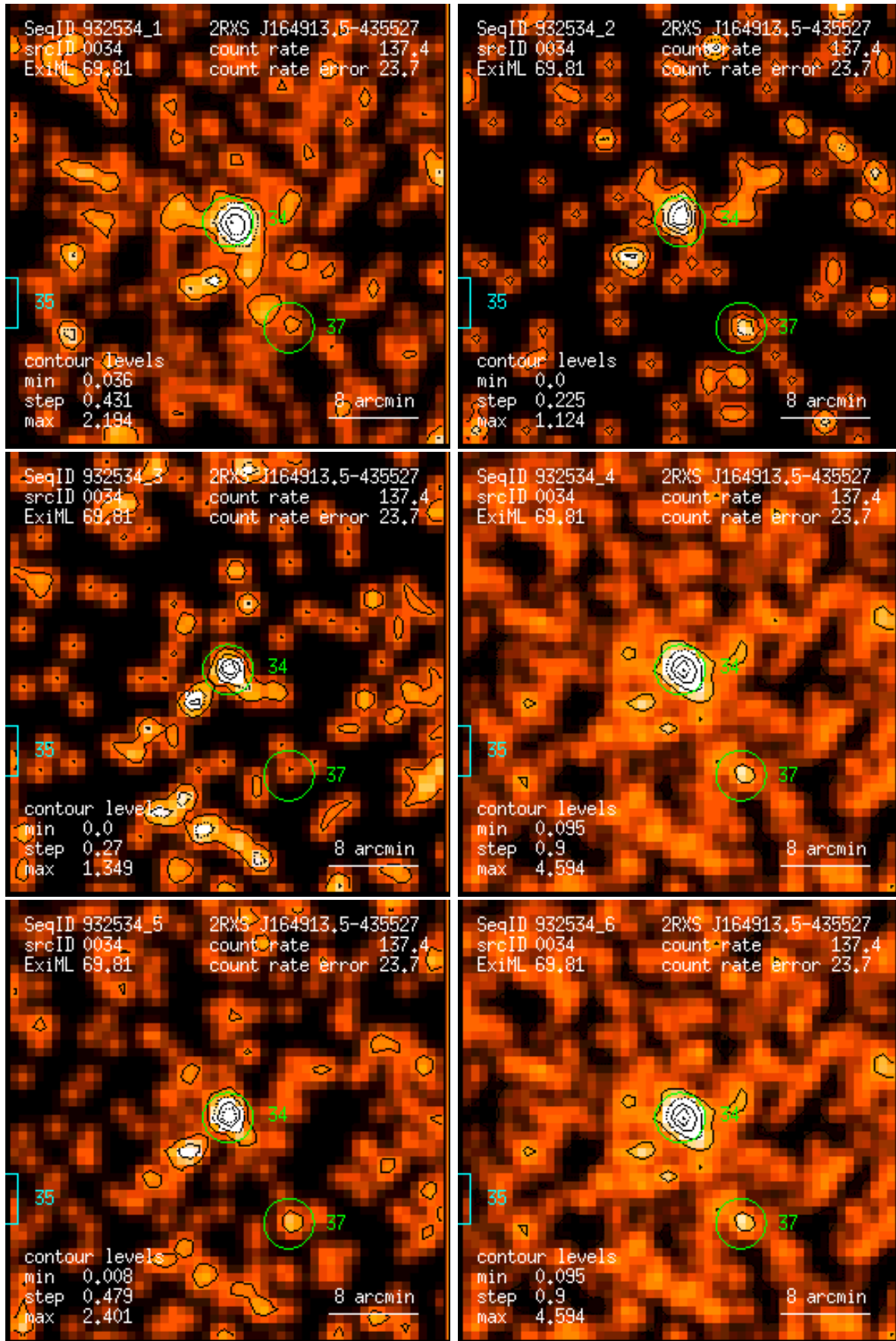
Figure 34: RASS 932534: detection 0034: band rate images, Gaussian filter: (1) PSPC channels 11 – 41, (2) 52 – 90, (3) 91 – 201, (4) 11 – 235, (5) 52 – 201, (6) 11 – 201. Broad band rates in counts/ks. Band rate contour levels in counts/ks/arcmin 2 .
