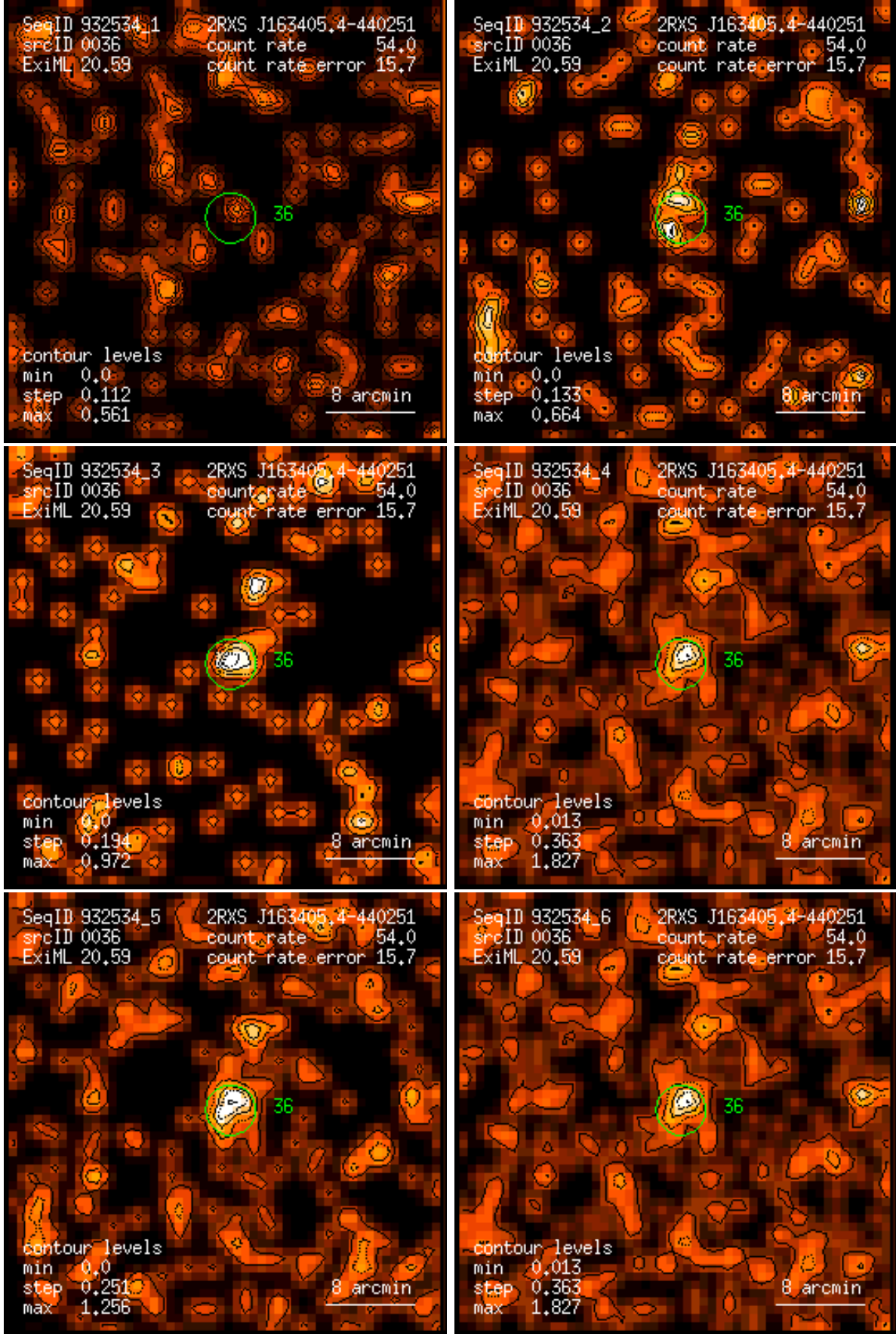
Figure 36: RASS 932534: detection 0036: band rate images, Gaussian filter: (1) PSPC channels 11 – 41, (2) 52 – 90, (3) 91 – 201, (4) 11 – 235, (5) 52 – 201, (6) 11 – 201. Broad band rates in counts/ks. Band rate contour levels in counts/ks/arcmin 2 .
