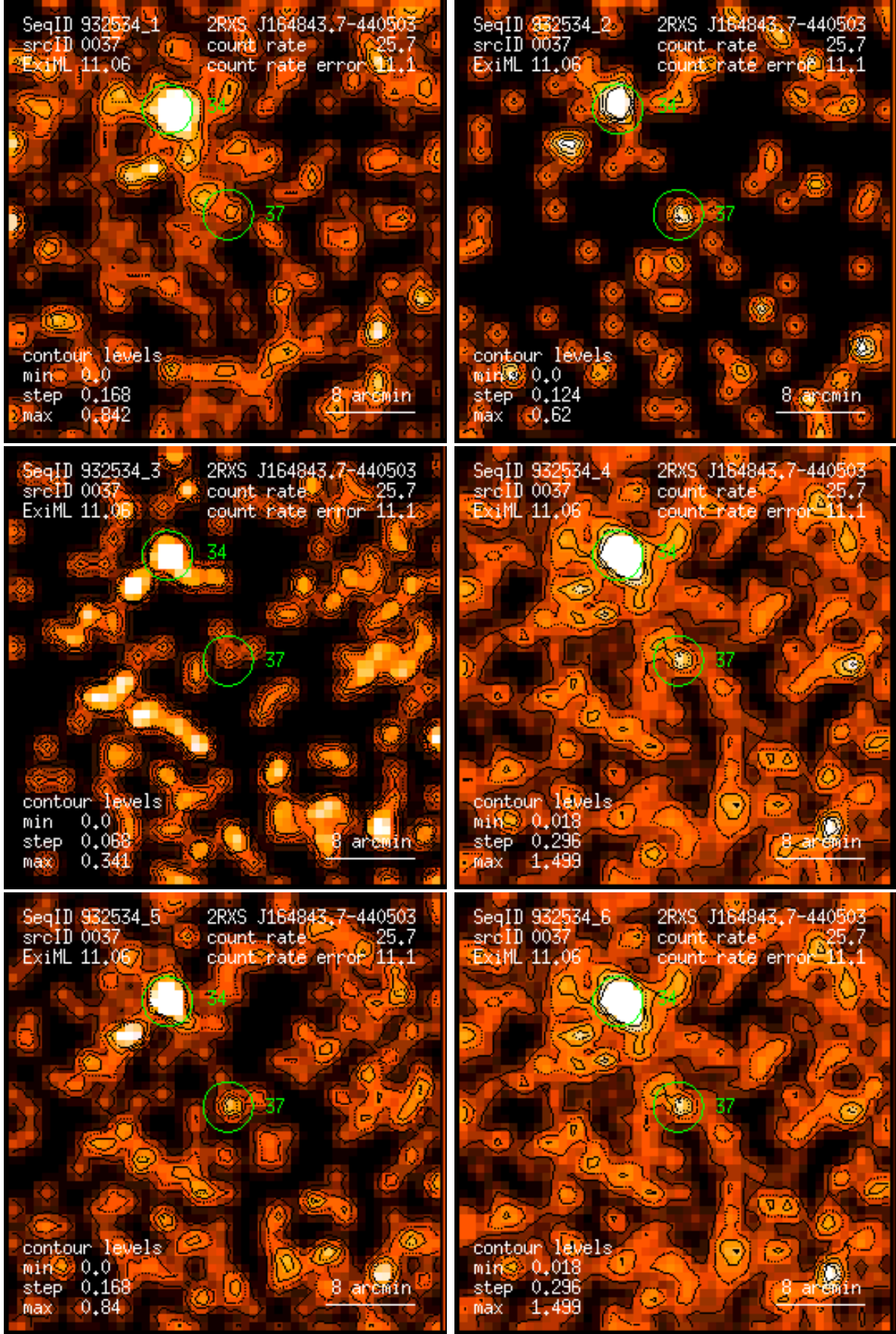
Figure 37: RASS 932534: detection 0037: band rate images, Gaussian filter: (1) PSPC channels 11 – 41, (2) 52 – 90, (3) 91 – 201, (4) 11 – 235, (5) 52 – 201, (6) 11 – 201. Broad band rates in counts/ks. Band rate contour levels in counts/ks/arcmin 2 .
