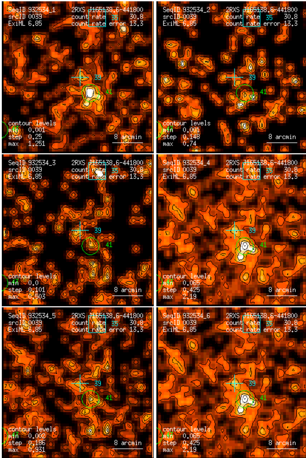
Figure 39: RASS 932534: detection 0039: band rate images, Gaussian filter: (1) PSPC channels 11 – 41, (2) 52 – 90, (3) 91 – 201, (4) 11 – 235, (5) 52 – 201, (6) 11 – 201. Broad band rates in counts/ks. Band rate contour levels in counts/ks/arcmin 2 .
