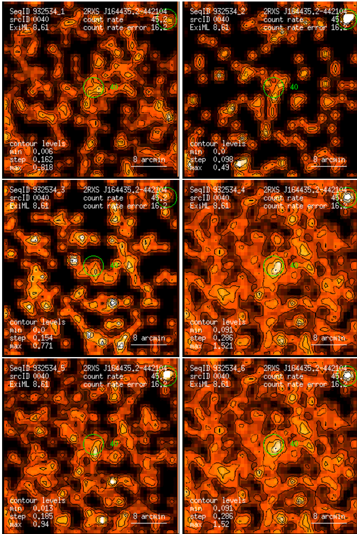
Figure 40: RASS 932534: detection 0040: band rate images, Gaussian filter: (1) PSPC channels 11 – 41, (2) 52 – 90, (3) 91 – 201, (4) 11 – 235, (5) 52 – 201, (6) 11 – 201. Broad band rates in counts/ks. Band rate contour levels in counts/ks/arcmin 2 .
