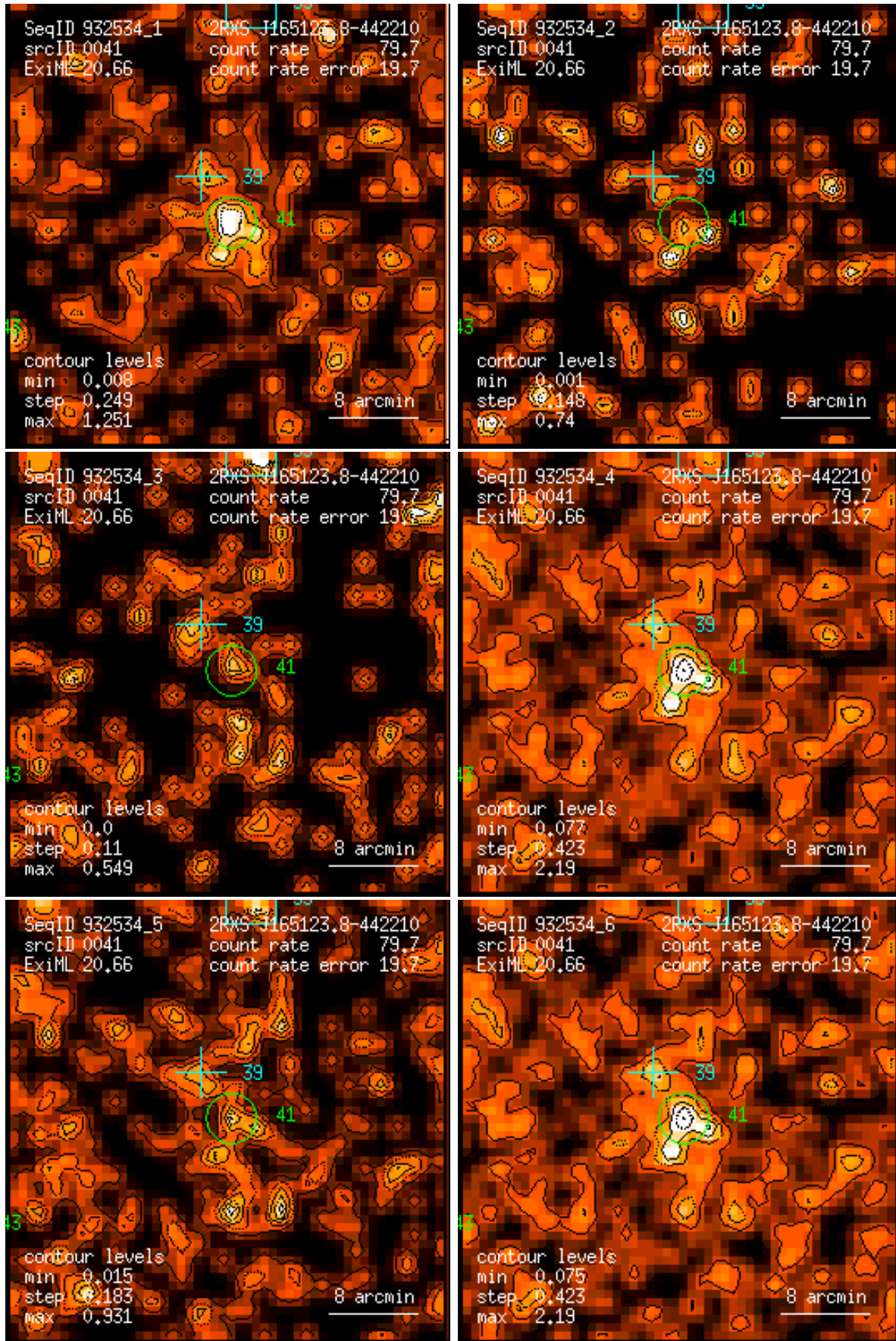
Figure 41: RASS 932534: detection 0041: band rate images, Gaussian filter: (1) PSPC channels 11 – 41, (2) 52 – 90, (3) 91 – 201, (4) 11 – 235, (5) 52 – 201, (6) 11 – 201. Broad band rates in counts/ks. Band rate contour levels in counts/ks/arcmin 2 .
