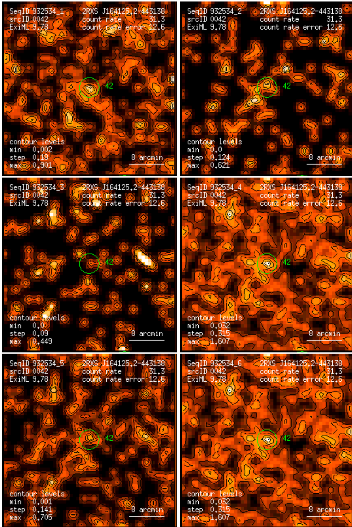
Figure 42: RASS 932534: detection 0042: band rate images, Gaussian filter: (1) PSPC channels 11 – 41, (2) 52 – 90, (3) 91 – 201, (4) 11 – 235, (5) 52 – 201, (6) 11 – 201. Broad band rates in counts/ks. Band rate contour levels in counts/ks/arcmin 2 .
