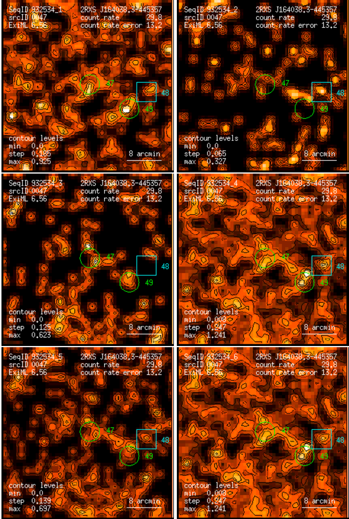
Figure 47: RASS 932534: detection 0047: band rate images, Gaussian filter: (1) PSPC channels 11 – 41, (2) 52 – 90, (3) 91 – 201, (4) 11 – 235, (5) 52 – 201, (6) 11 – 201. Broad band rates in counts/ks. Band rate contour levels in counts/ks/arcmin 2 .
