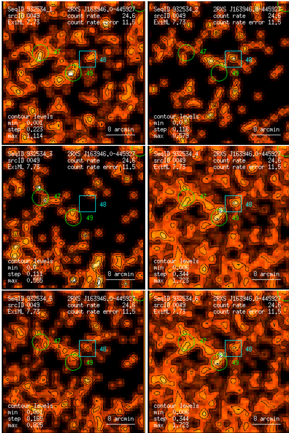
Figure 49: RASS 932534: detection 0049: band rate images, Gaussian filter: (1) PSPC channels 11 – 41, (2) 52 – 90, (3) 91 – 201, (4) 11 – 235, (5) 52 – 201, (6) 11 – 201. Broad band rates in counts/ks. Band rate contour levels in counts/ks/arcmin 2 .
