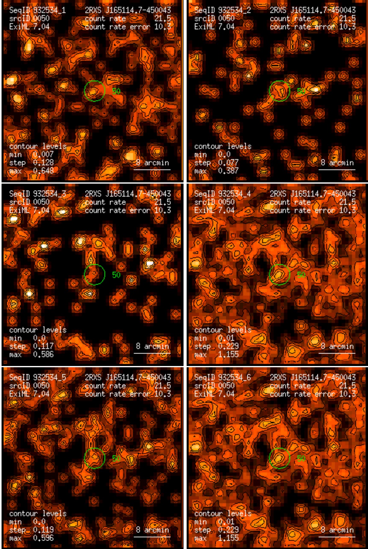
Figure 50: RASS 932534: detection 0050: band rate images, Gaussian filter: (1) PSPC channels 11 – 41, (2) 52 – 90, (3) 91 – 201, (4) 11 – 235, (5) 52 – 201, (6) 11 – 201. Broad band rates in counts/ks. Band rate contour levels in counts/ks/arcmin 2 .
