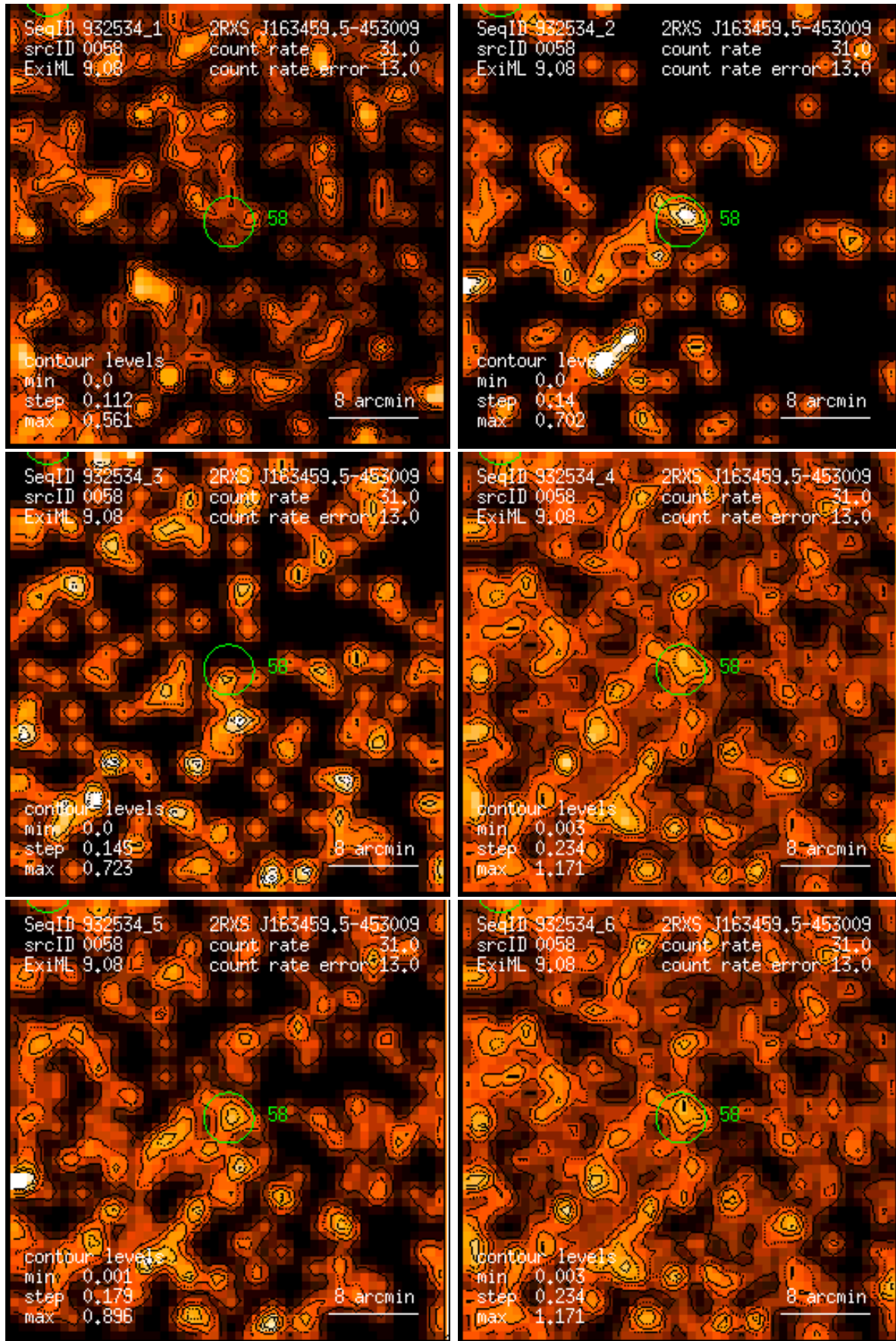
Figure 58: RASS 932534: detection 0058: band rate images, Gaussian filter: (1) PSPC channels 11 – 41, (2) 52 – 90, (3) 91 – 201, (4) 11 – 235, (5) 52 – 201, (6) 11 – 201. Broad band rates in counts/ks. Band rate contour levels in counts/ks/arcmin 2 .
