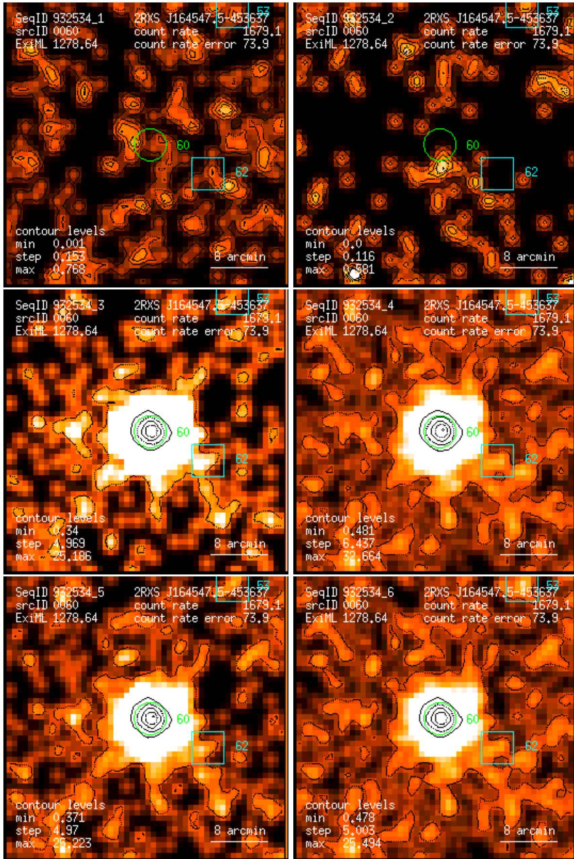
Figure 60: RASS 932534: detection 0060: band rate images, Gaussian filter: (1) PSPC channels 11 – 41, (2) 52 – 90, (3) 91 – 201, (4) 11 – 235, (5) 52 – 201, (6) 11 – 201. Broad band rates in counts/ks. Band rate contour levels in counts/ks/arcmin 2 .
