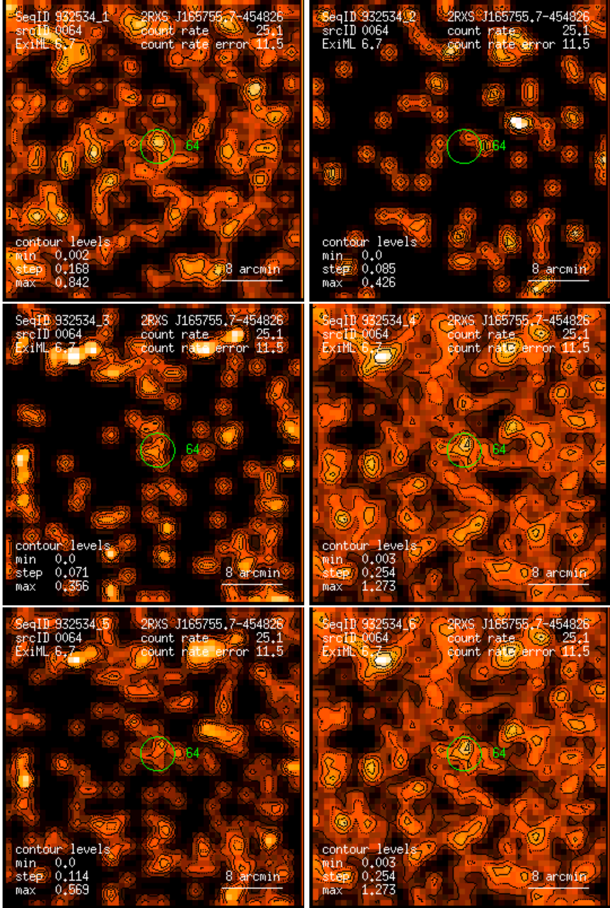
Figure 64: RASS 932534: detection 0064: band rate images, Gaussian filter: (1) PSPC channels 11 – 41, (2) 52 – 90, (3) 91 – 201, (4) 11 – 235, (5) 52 – 201, (6) 11 – 201. Broad band rates in counts/ks. Band rate contour levels in counts/ks/arcmin 2 .
