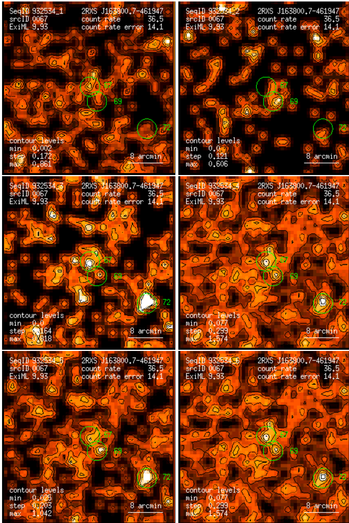
Figure 67: RASS 932534: detection 0067: band rate images, Gaussian filter: (1) PSPC channels 11 – 41, (2) 52 – 90, (3) 91 – 201, (4) 11 – 235, (5) 52 – 201, (6) 11 – 201. Broad band rates in counts/ks. Band rate contour levels in counts/ks/arcmin 2 .
