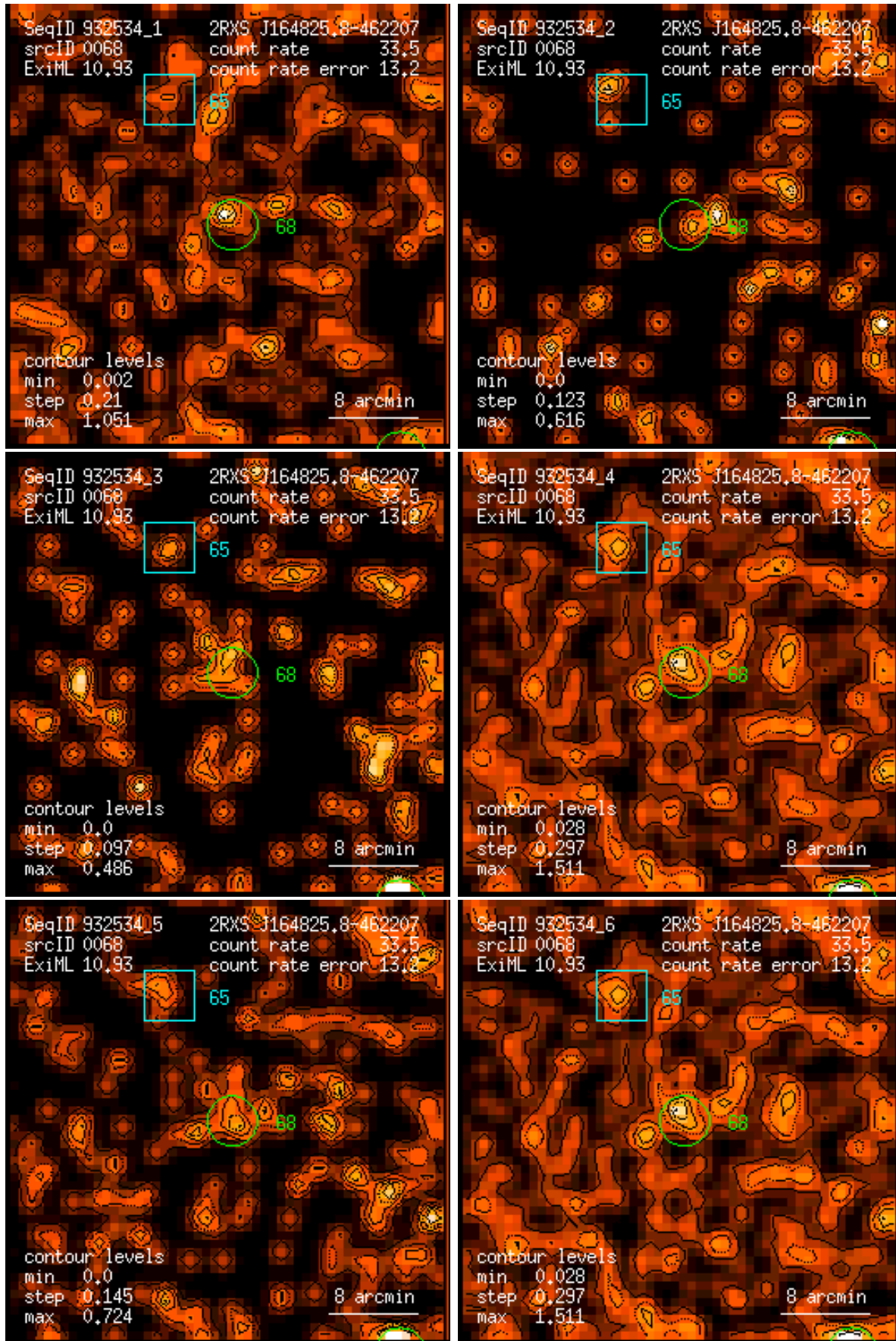
Figure 68: RASS 932534: detection 0068: band rate images, Gaussian filter: (1) PSPC channels 11 – 41, (2) 52 – 90, (3) 91 – 201, (4) 11 – 235, (5) 52 – 201, (6) 11 – 201. Broad band rates in counts/ks. Band rate contour levels in counts/ks/arcmin 2 .
