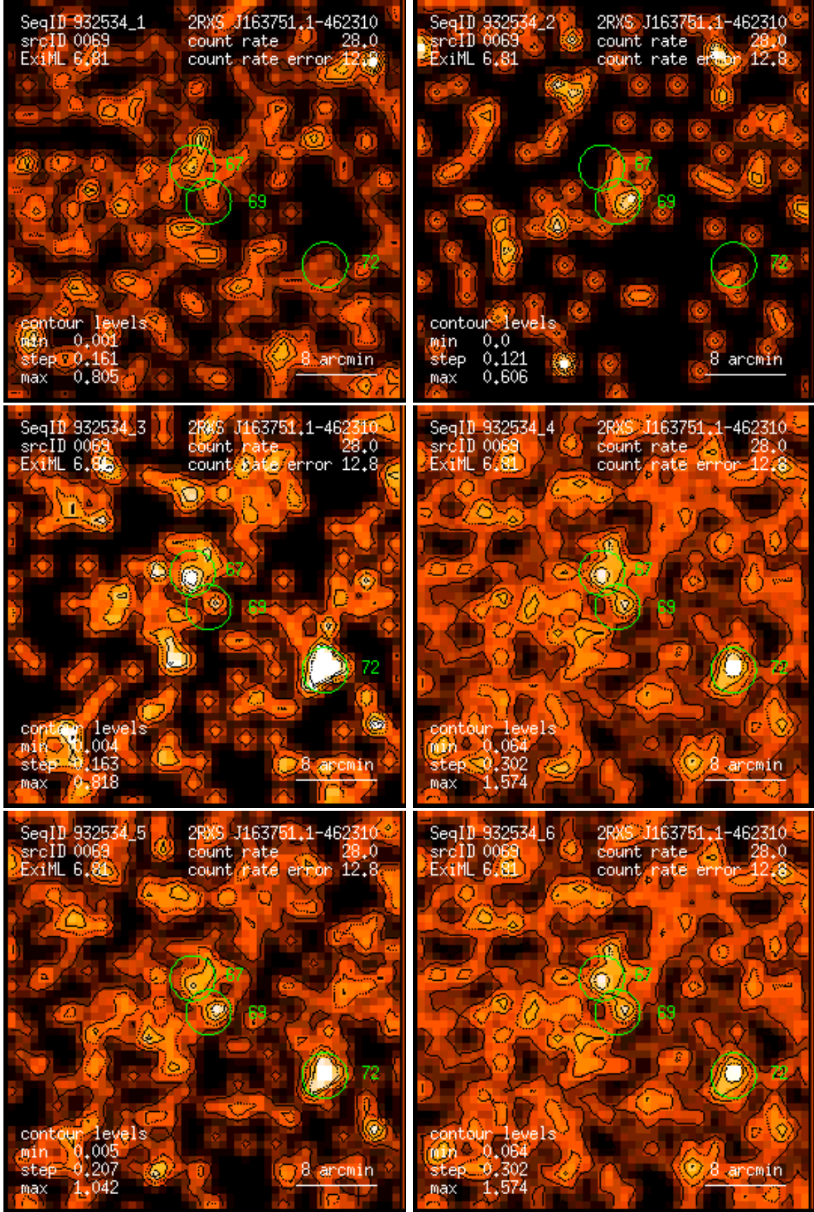
Figure 69: RASS 932534: detection 0069: band rate images, Gaussian filter: (1) PSPC channels 11 – 41, (2) 52 – 90, (3) 91 – 201, (4) 11 – 235, (5) 52 – 201, (6) 11 – 201. Broad band rates in counts/ks. Band rate contour levels in counts/ks/arcmin 2 .
