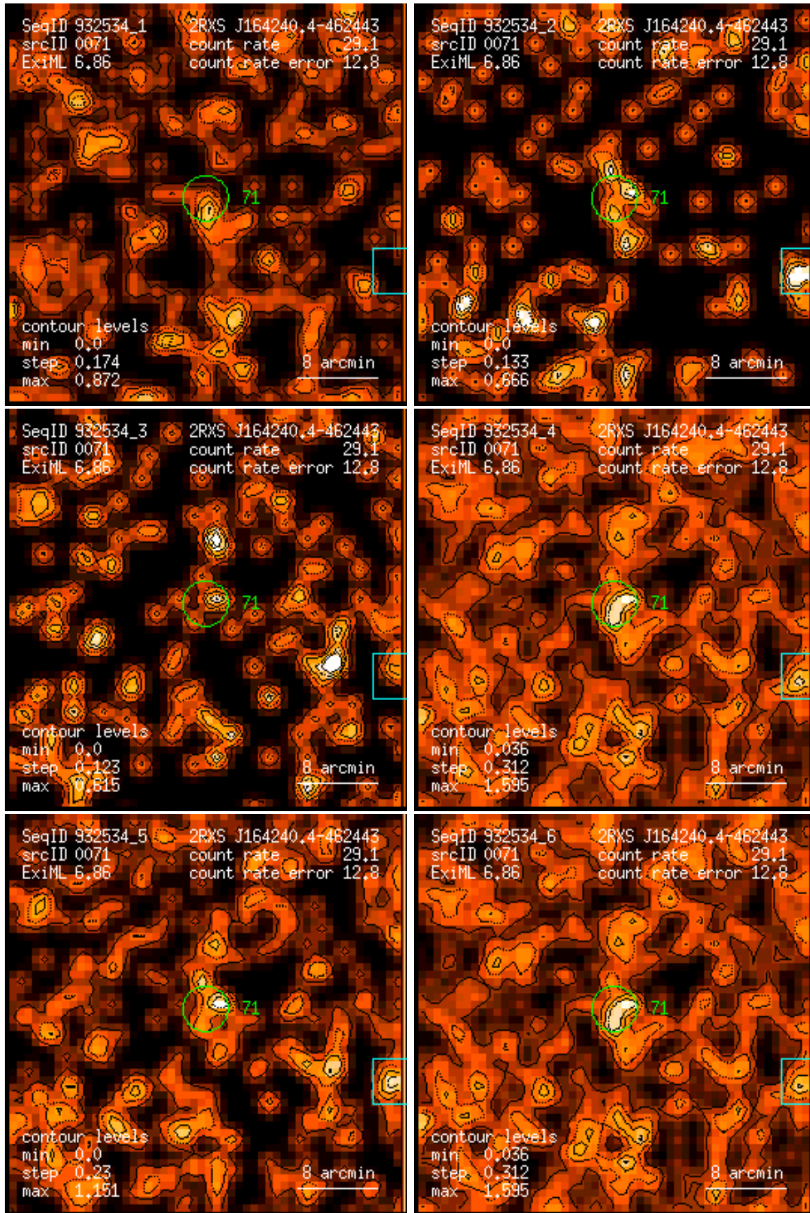
Figure 71: RASS 932534: detection 0071: band rate images, Gaussian filter: (1) PSPC channels 11 – 41, (2) 52 – 90, (3) 91 – 201, (4) 11 – 235, (5) 52 – 201, (6) 11 – 201. Broad band rates in counts/ks. Band rate contour levels in counts/ks/arcmin 2 .
