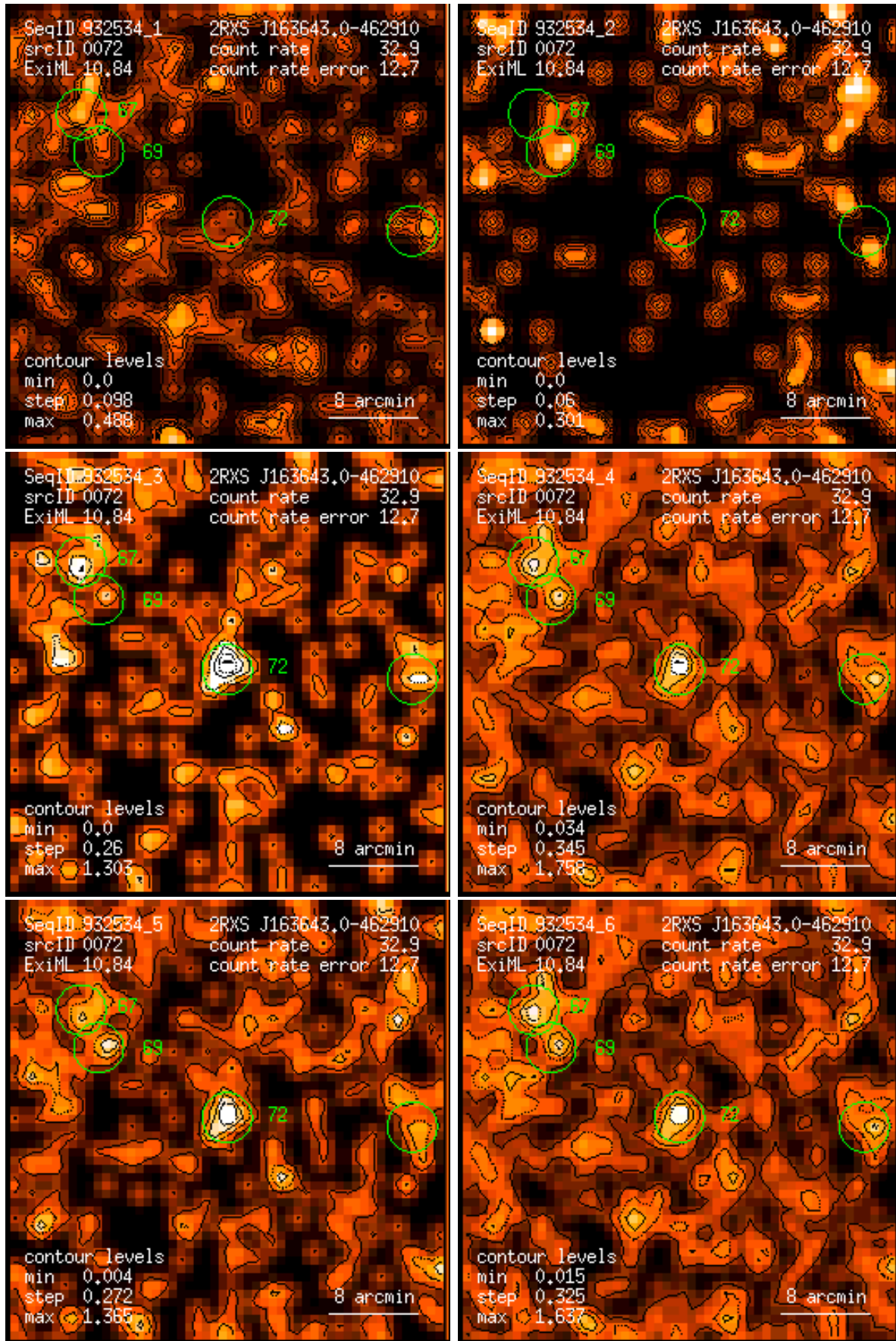
Figure 72: RASS 932534: detection 0072: band rate images, Gaussian filter: (1) PSPC channels 11 – 41, (2) 52 – 90, (3) 91 – 201, (4) 11 – 235, (5) 52 – 201, (6) 11 – 201. Broad band rates in counts/ks. Band rate contour levels in counts/ks/arcmin 2 .
