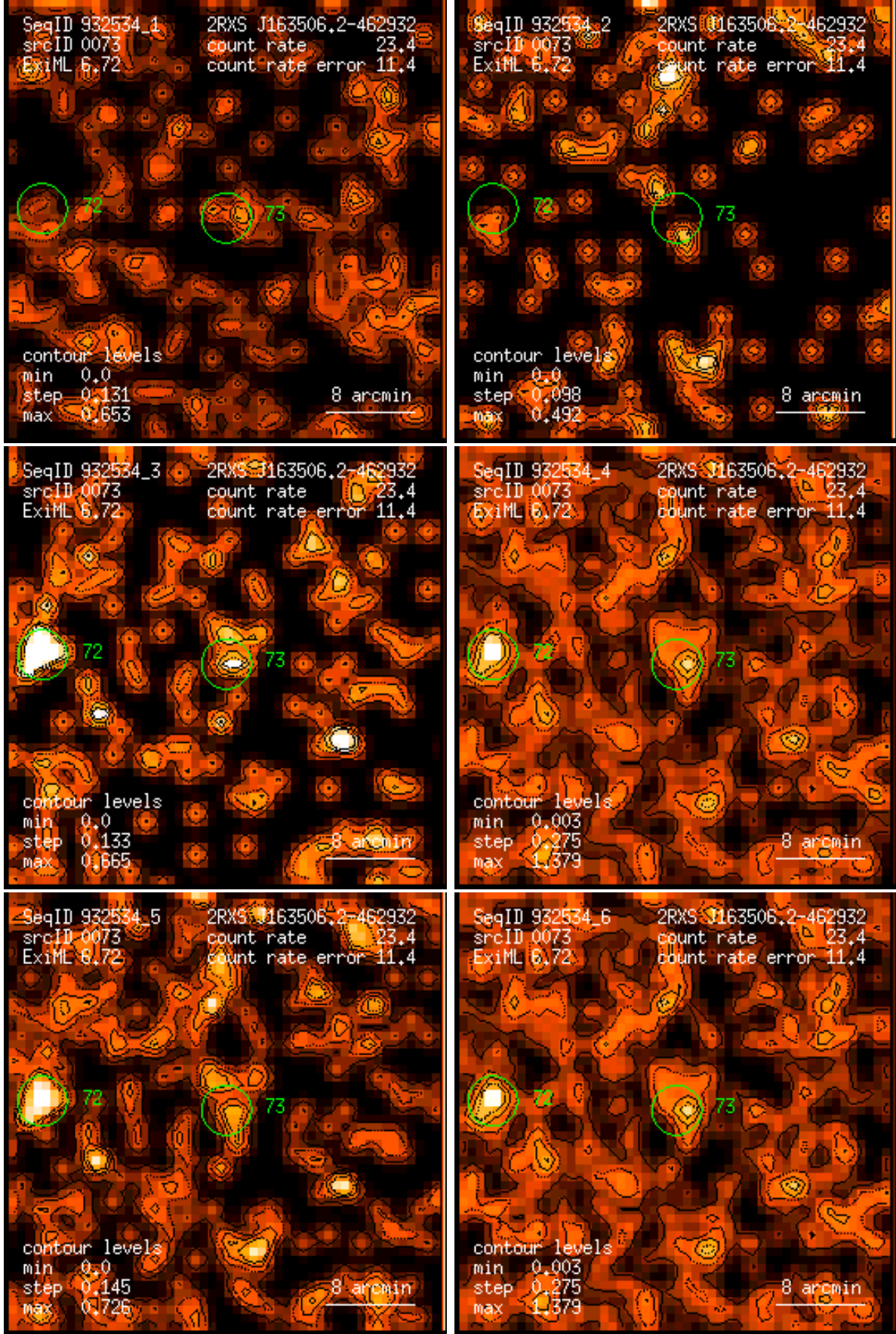
Figure 73: RASS 932534: detection 0073: band rate images, Gaussian filter: (1) PSPC channels 11 – 41, (2) 52 – 90, (3) 91 – 201, (4) 11 – 235, (5) 52 – 201, (6) 11 – 201. Broad band rates in counts/ks. Band rate contour levels in counts/ks/arcmin 2 .
