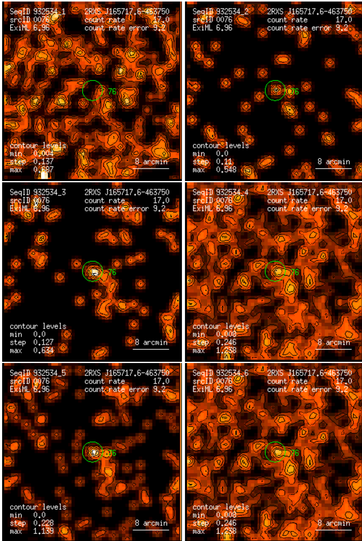
Figure 76: RASS 932534: detection 0076: band rate images, Gaussian filter: (1) PSPC channels 11 – 41, (2) 52 – 90, (3) 91 – 201, (4) 11 – 235, (5) 52 – 201, (6) 11 – 201. Broad band rates in counts/ks. Band rate contour levels in counts/ks/arcmin 2 .
