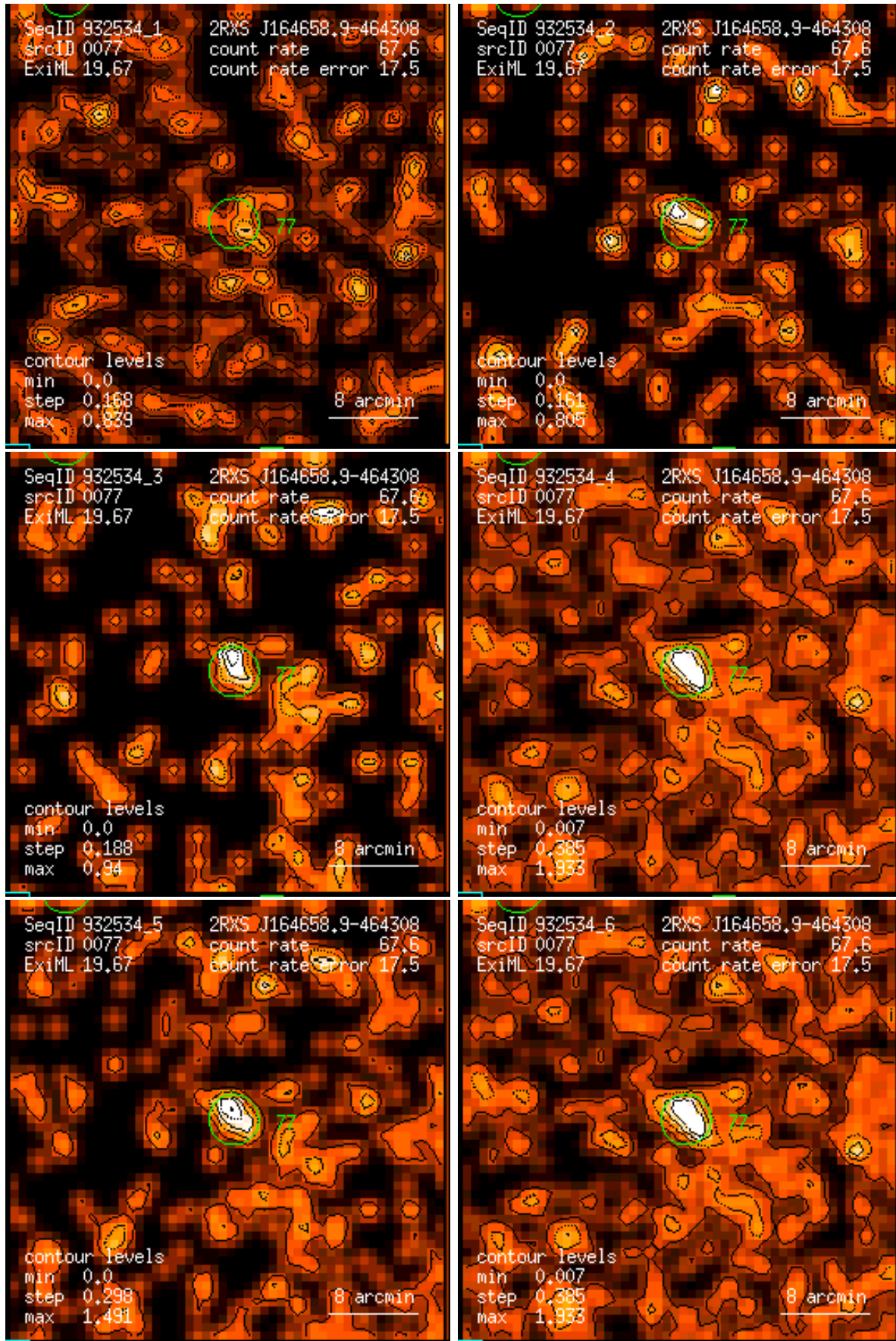
Figure 77: RASS 932534: detection 0077: band rate images, Gaussian filter: (1) PSPC channels 11 – 41, (2) 52 – 90, (3) 91 – 201, (4) 11 – 235, (5) 52 – 201, (6) 11 – 201. Broad band rates in counts/ks. Band rate contour levels in counts/ks/arcmin 2 .
