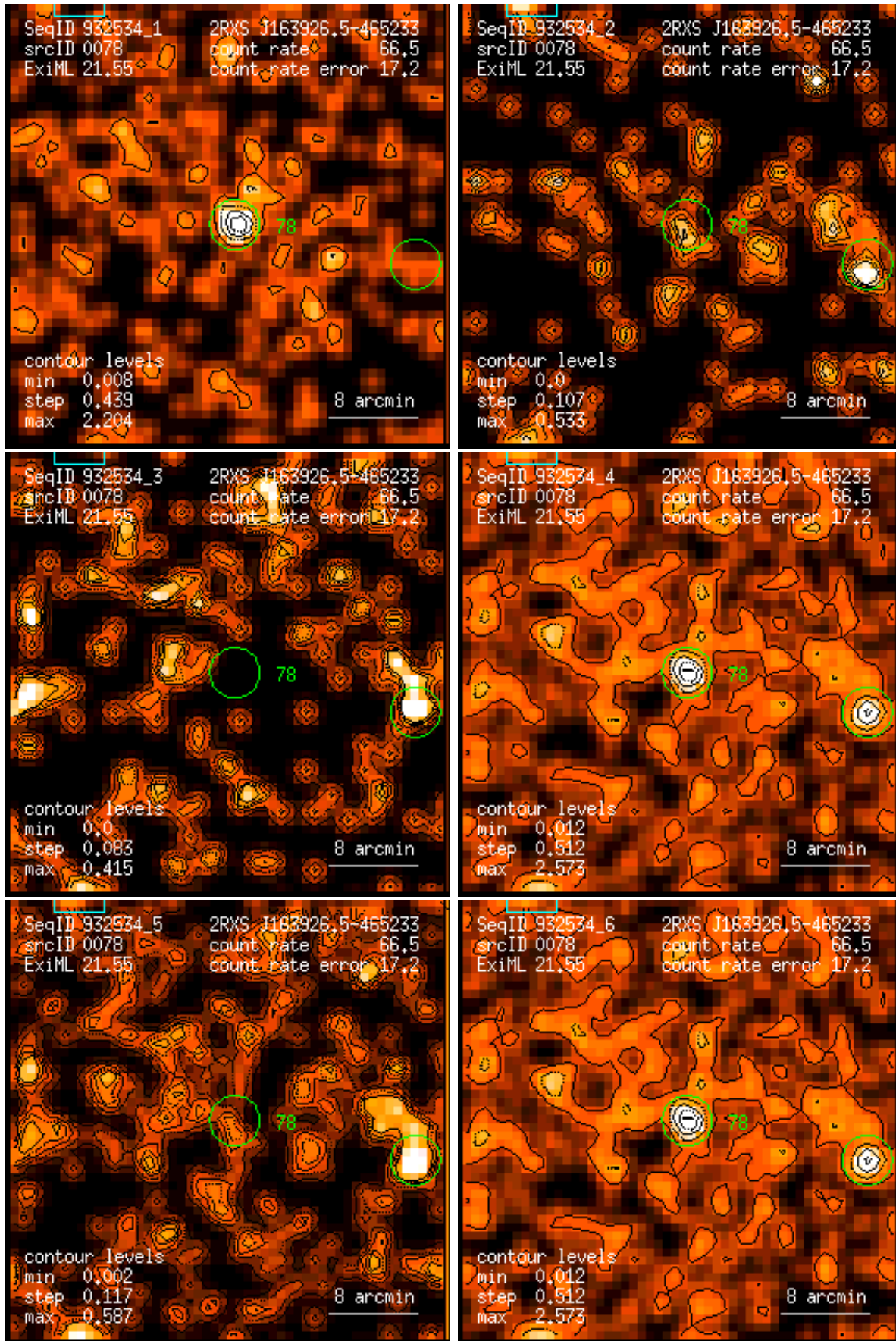
Figure 78: RASS 932534: detection 0078: band rate images, Gaussian filter: (1) PSPC channels 11 – 41, (2) 52 – 90, (3) 91 – 201, (4) 11 – 235, (5) 52 – 201, (6) 11 – 201. Broad band rates in counts/ks. Band rate contour levels in counts/ks/arcmin 2 .
