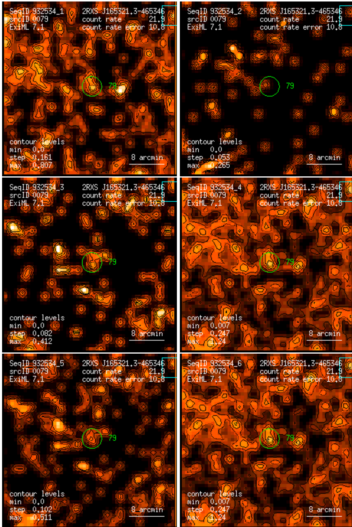
Figure 79: RASS 932534: detection 0079: band rate images, Gaussian filter: (1) PSPC channels 11 – 41, (2) 52 – 90, (3) 91 – 201, (4) 11 – 235, (5) 52 – 201, (6) 11 – 201. Broad band rates in counts/ks. Band rate contour levels in counts/ks/arcmin 2 .
