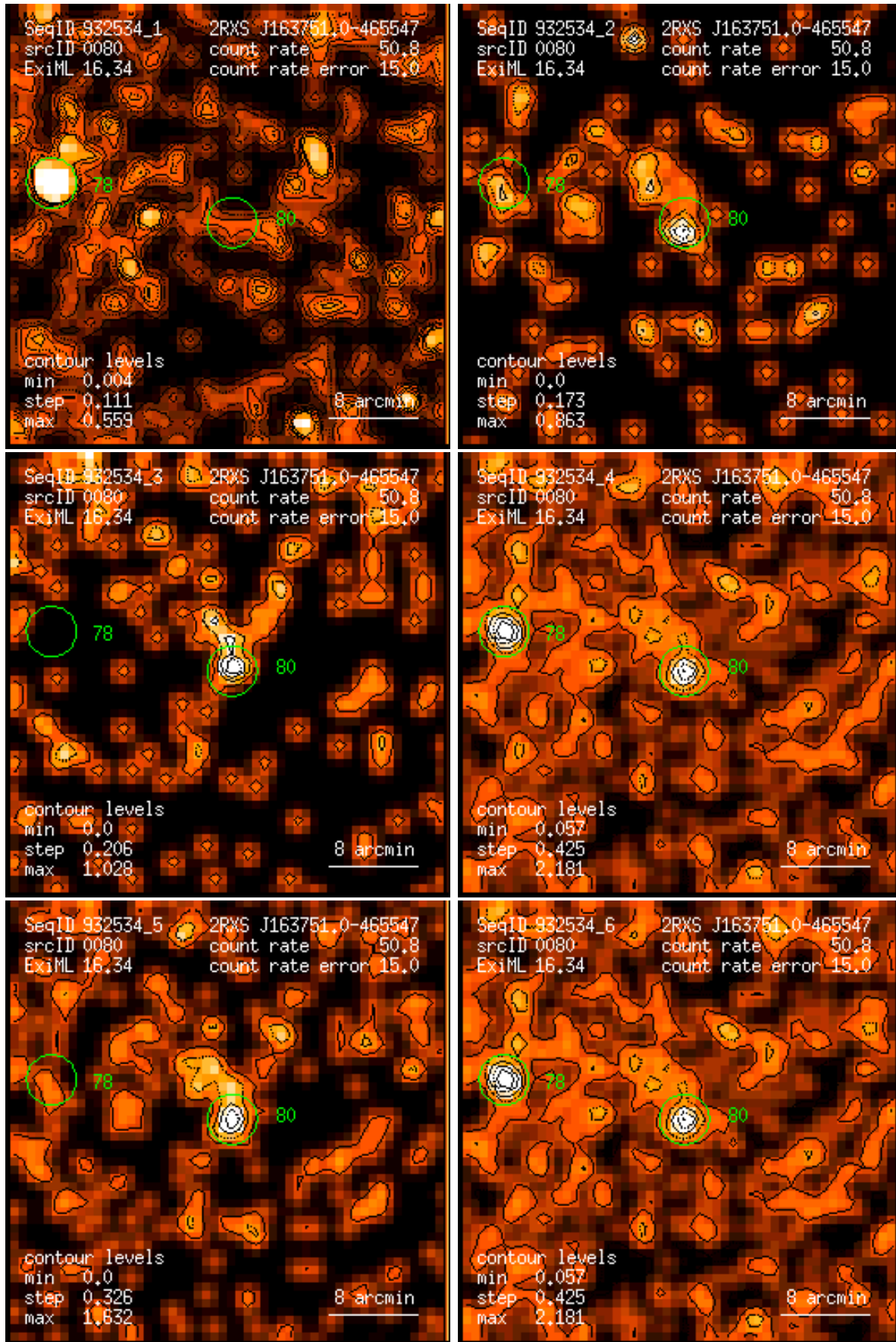
Figure 80: RASS 932534: detection 0080: band rate images, Gaussian filter: (1) PSPC channels 11 – 41, (2) 52 – 90, (3) 91 – 201, (4) 11 – 235, (5) 52 – 201, (6) 11 – 201. Broad band rates in counts/ks. Band rate contour levels in counts/ks/arcmin 2 .
