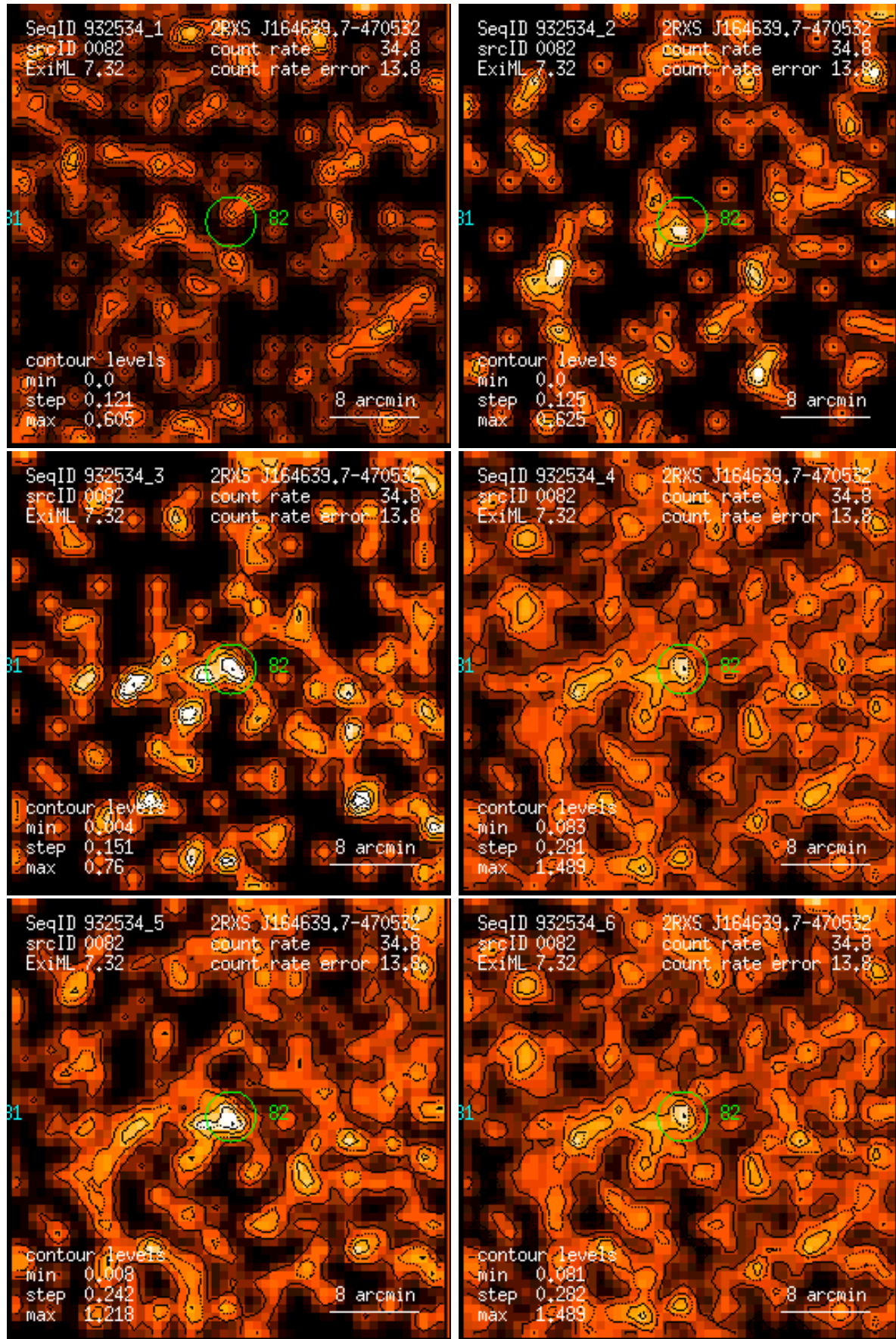
Figure 82: RASS 932534: detection 0082: band rate images, Gaussian filter: (1) PSPC channels 11 – 41, (2) 52 – 90, (3) 91 – 201, (4) 11 – 235, (5) 52 – 201, (6) 11 – 201. Broad band rates in counts/ks. Band rate contour levels in counts/ks/arcmin 2 .
