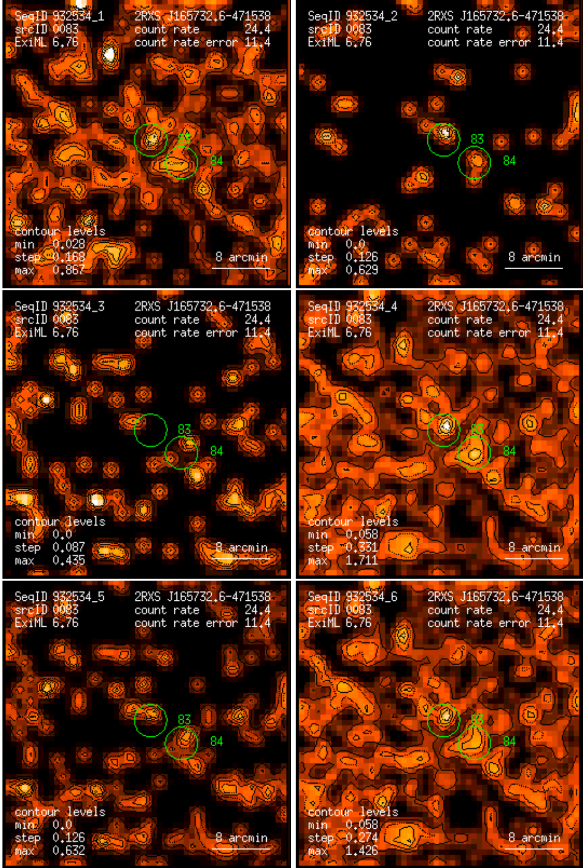
Figure 83: RASS 932534: detection 0083: band rate images, Gaussian filter: (1) PSPC channels 11 – 41, (2) 52 – 90, (3) 91 – 201, (4) 11 – 235, (5) 52 – 201, (6) 11 – 201. Broad band rates in counts/ks. Band rate contour levels in counts/ks/arcmin 2 .
