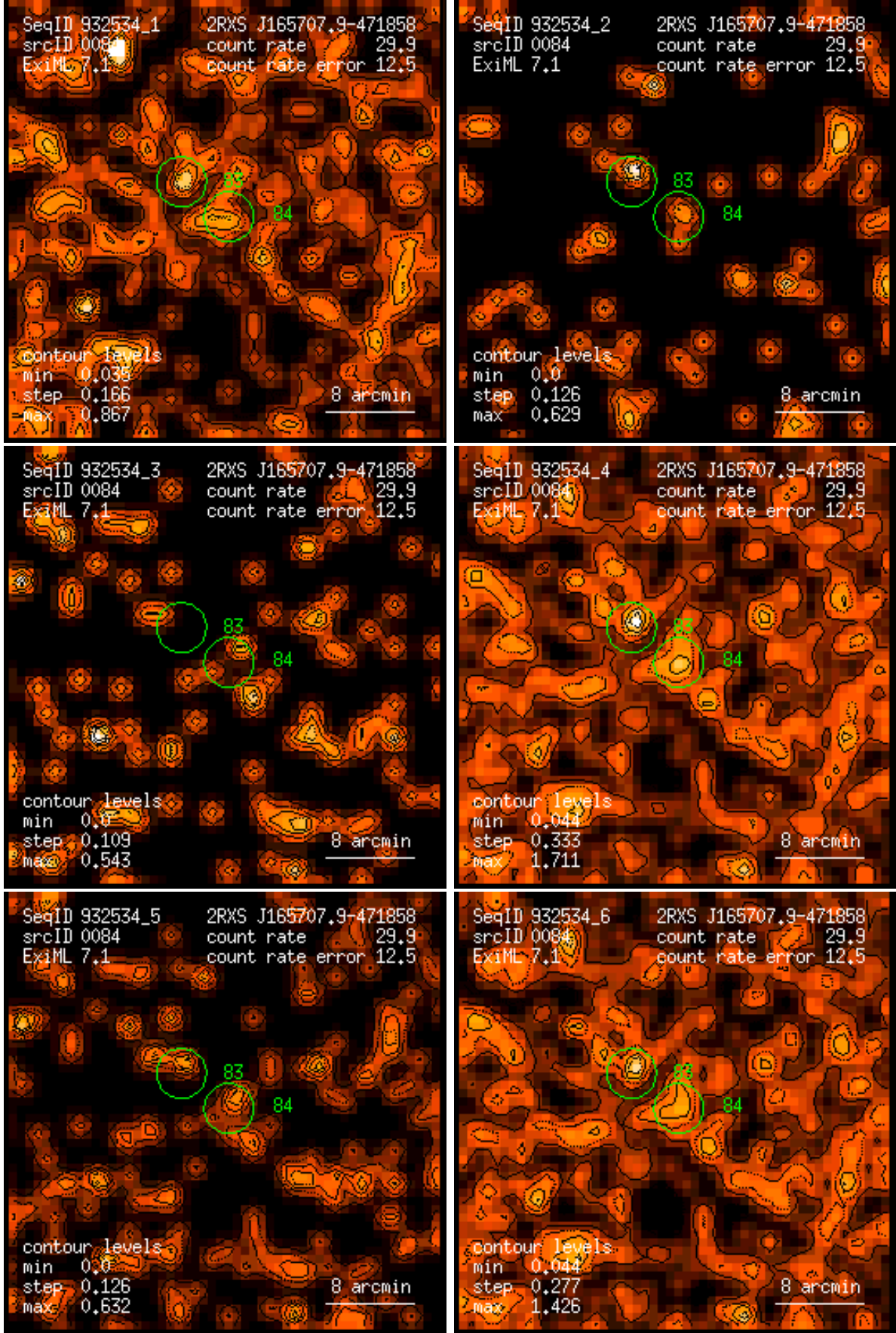
Figure 84: RASS 932534: detection 0084: band rate images, Gaussian filter: (1) PSPC channels 11 – 41, (2) 52 – 90, (3) 91 – 201, (4) 11 – 235, (5) 52 – 201, (6) 11 – 201. Broad band rates in counts/ks. Band rate contour levels in counts/ks/arcmin 2 .
